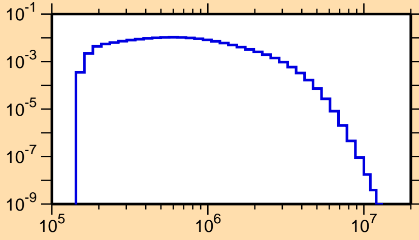
\sigma vs. E for ^{189}\text{Hg}(n,n_3)
