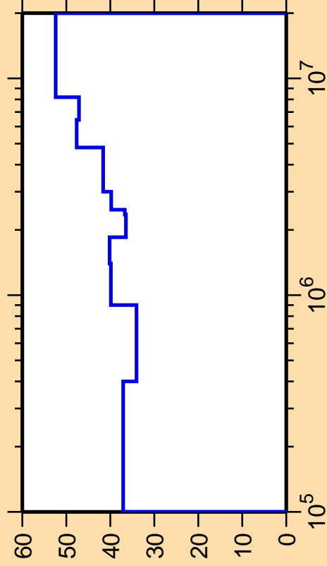
\Delta\sigma/\sigma vs. E for ^{189}\text{Hg}(n,n_4)
