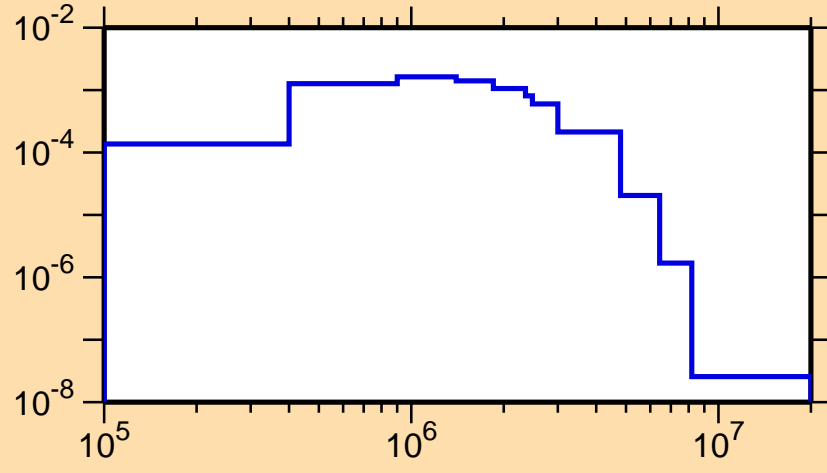
\sigma vs. E for ^{189}\text{Hg}(n,n_4)
