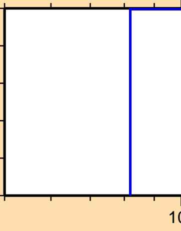
\sigma vs. E for ^{191}\text{Hg}(n,\text{He}3)
