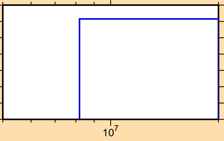
\sigma vs. E for ^{191}\text{Hg}(n,nt)
