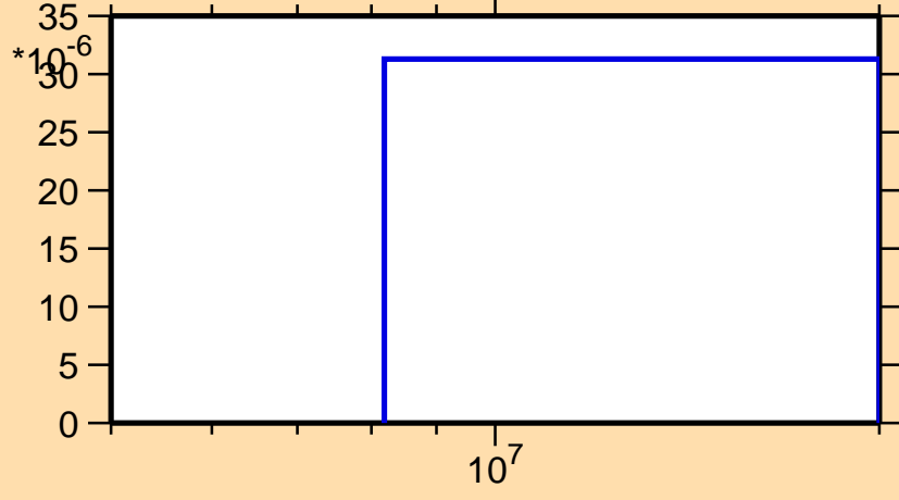
\sigma vs. E for ^{192}\text{Hg}(n,3n)
