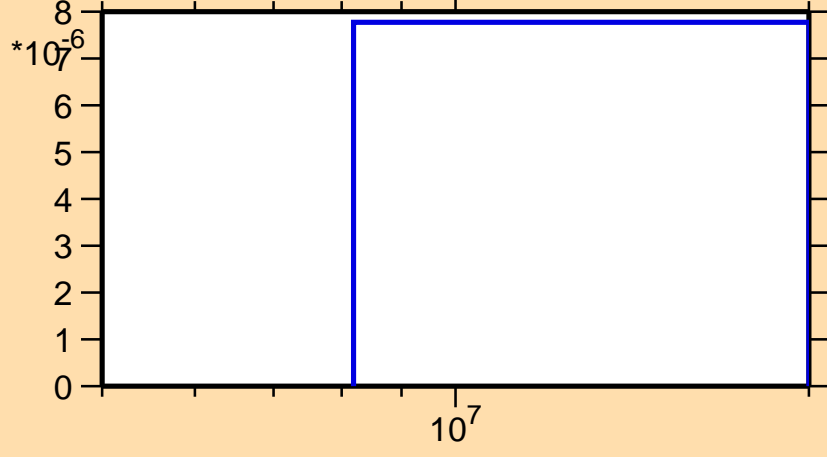
\sigma vs. E for ^{192}\text{Hg}(n,t)
