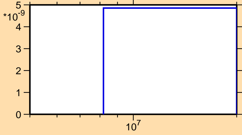
\sigma vs. E for ^{192}\text{Hg}(n,2n\alpha)
