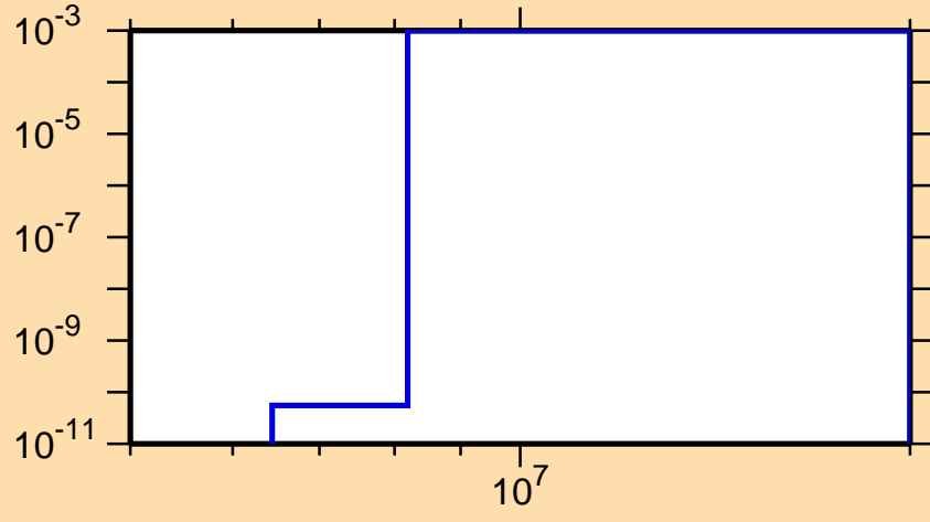
\sigma vs. E for ^{192}\text{Hg}(n,np)
