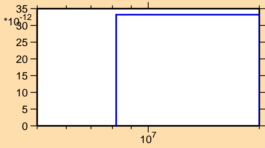
\sigma vs. E for ^{192}\text{Hg}(n,\text{nd})
