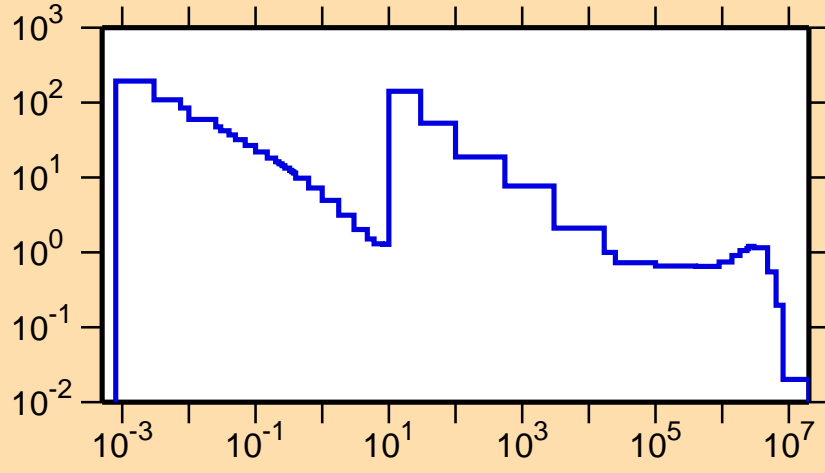
\sigma vs. E for ^{192}\text{Hg}(n,\gamma)
