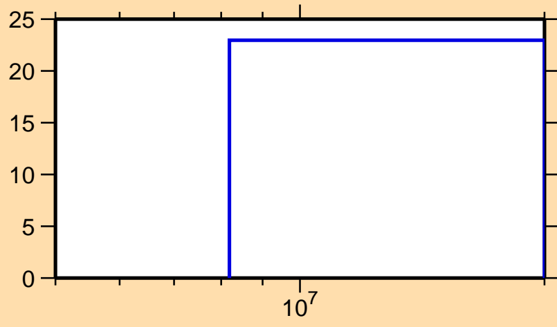
\Delta\sigma/\sigma vs. E for ^{192}\text{Hg}(n,\text{inel.})
