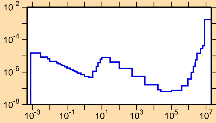
\sigma vs. E for ^{192}\text{Hg}(n,\alpha)
