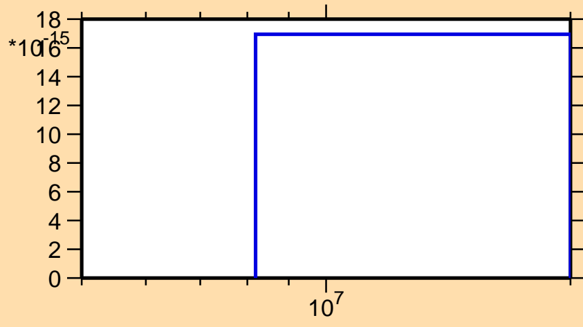
\sigma vs. E for ^{192}\text{Hg}(\text{mt117})
