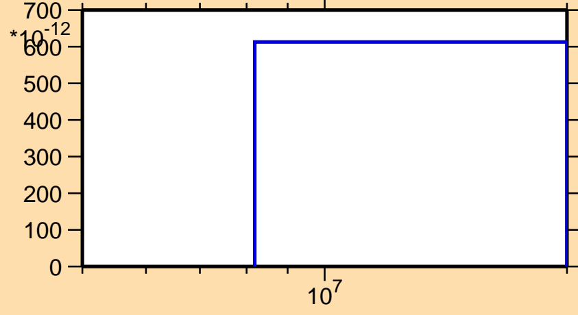
\sigma vs. E for ^{192}\text{Hg}(n,p\alpha)
