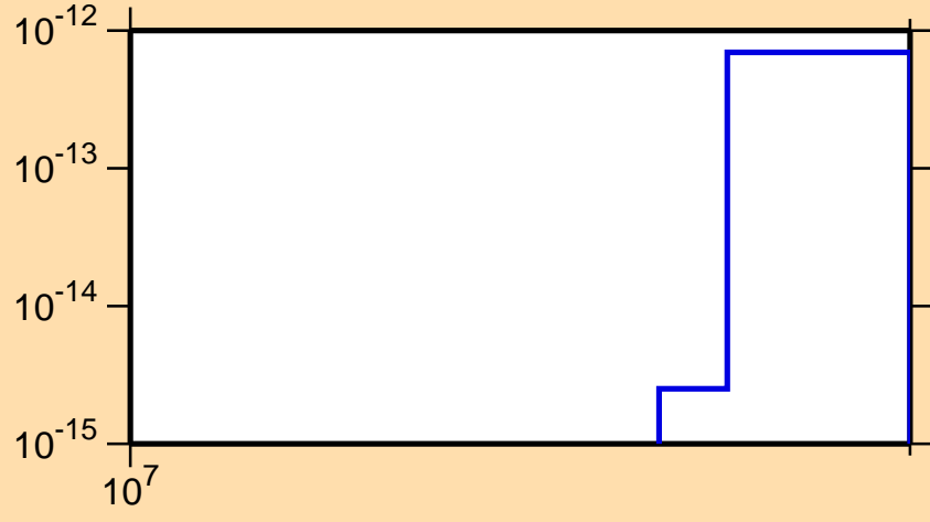
\sigma vs. E for ^{193}\text{Hg} (mt 34)
