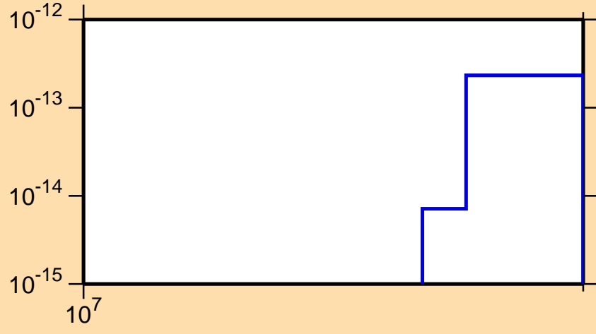
\sigma vs. E for ^{193}\text{Hg} (mt 45)
