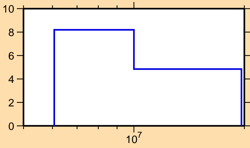
\Delta\sigma/\sigma vs. E for ^{193}\text{Hg}(n,\text{tot.})
