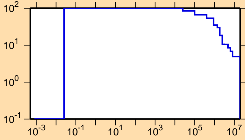
\Delta\sigma/\sigma vs. E for ^{193}\text{Hg}(n,\text{nonel.})
