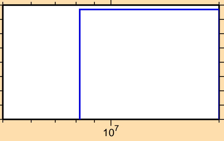
\sigma vs. E for ^{193}\text{Hg}(n,nt)
