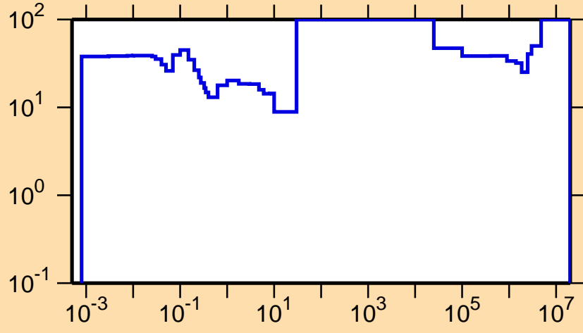
\Delta\sigma/\sigma vs. E for ^{193}\text{Hg}(n,\gamma)
