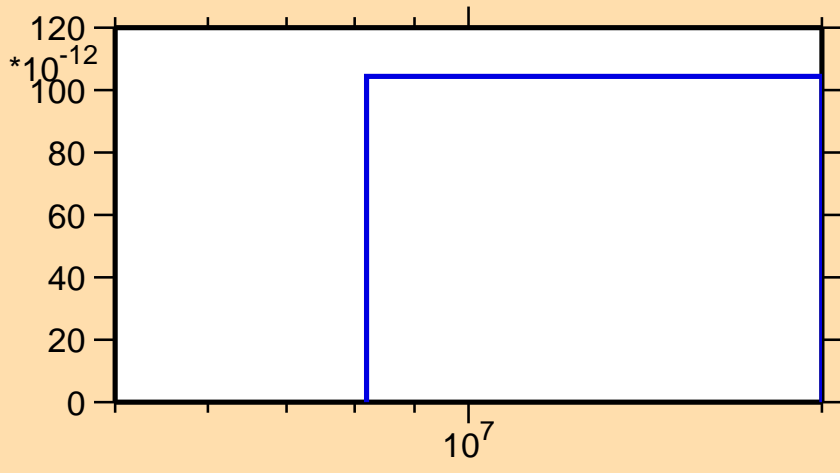
\sigma vs. E for ^{196}\text{Hg}(n,\text{nd})
