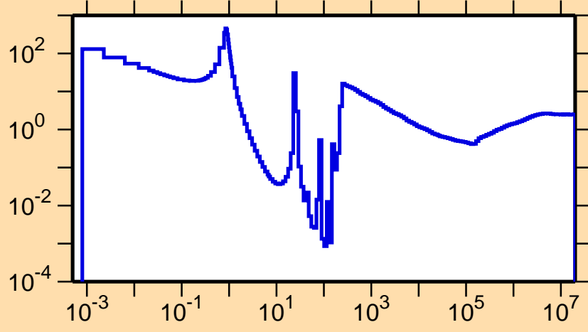
\sigma vs. E for ^{197}\text{Hg}(n,\text{nonel.})
