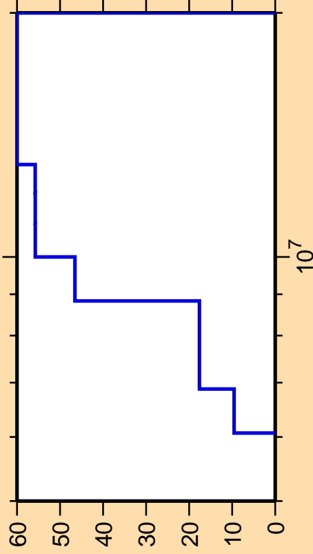
\Delta\sigma/\sigma vs. E for ^{197}\text{Hg}(n,n\text{cont.})
