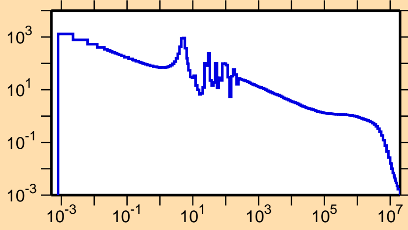
\sigma vs. E for ^{197}\text{Hg}(n,\gamma)
