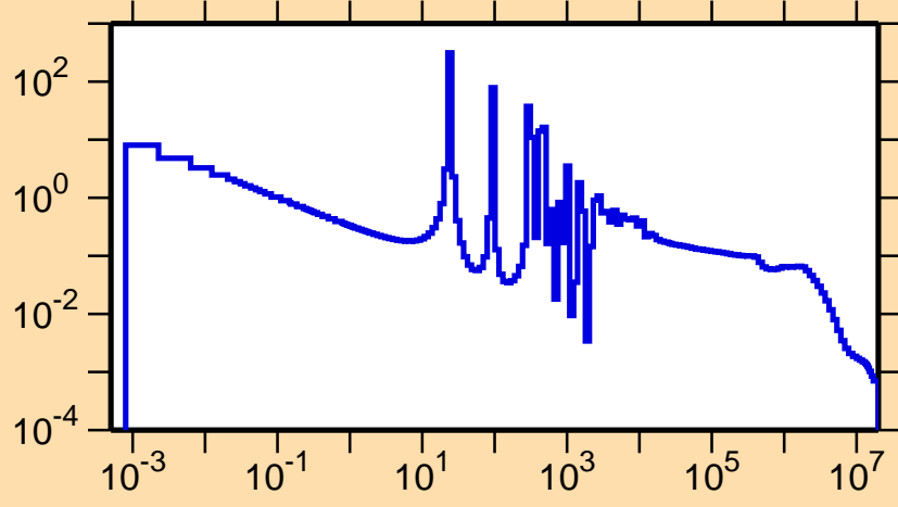
\sigma vs. E for ^{198}\text{Hg}(n,\gamma)
