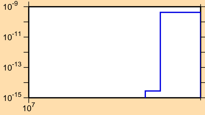
\sigma vs. E for ^{198}\text{Hg}(n,nt)
