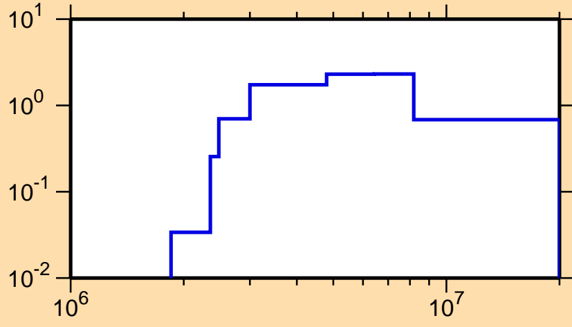
\sigma vs. E for ^{198}\text{Hg}(n,n\text{cont.})
