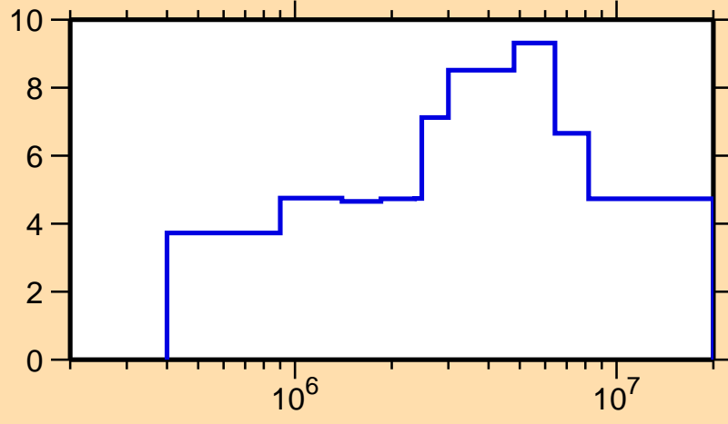
\Delta\sigma/\sigma vs. E for ^{198}\text{Hg}(n,\text{el.})
