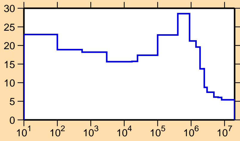
\Delta\sigma/\sigma vs. E for ^{198}\text{Hg}(n,\text{nonel.})
