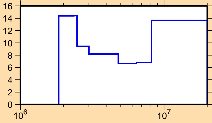
\Delta\sigma/\sigma vs. E for ^{198}\text{Hg}(n,\text{inel.})
