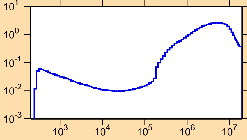
\sigma vs. E for ^{199}\text{Hg}(n,\text{inel.})
