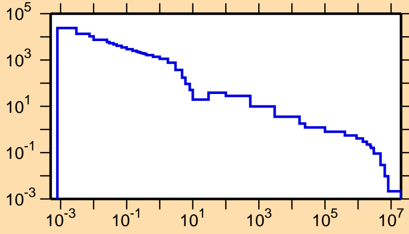
\sigma vs. E for ^{199}\text{Hg}(n,\gamma)
