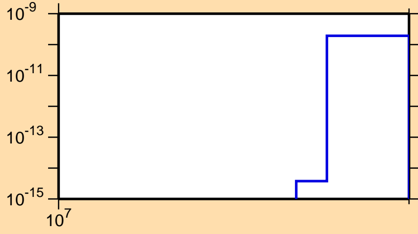
\sigma vs. E for ^{200}\text{Hg}(n,nt)
