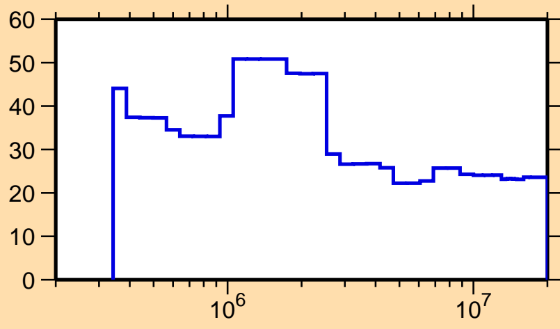
\Delta\sigma/\sigma vs. E for ^{200}\text{Hg}(n,n_1)
