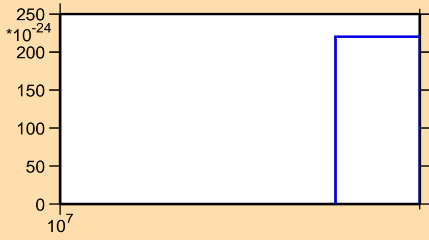
\sigma vs. E for ^{200}\text{Hg} (mt 11)
