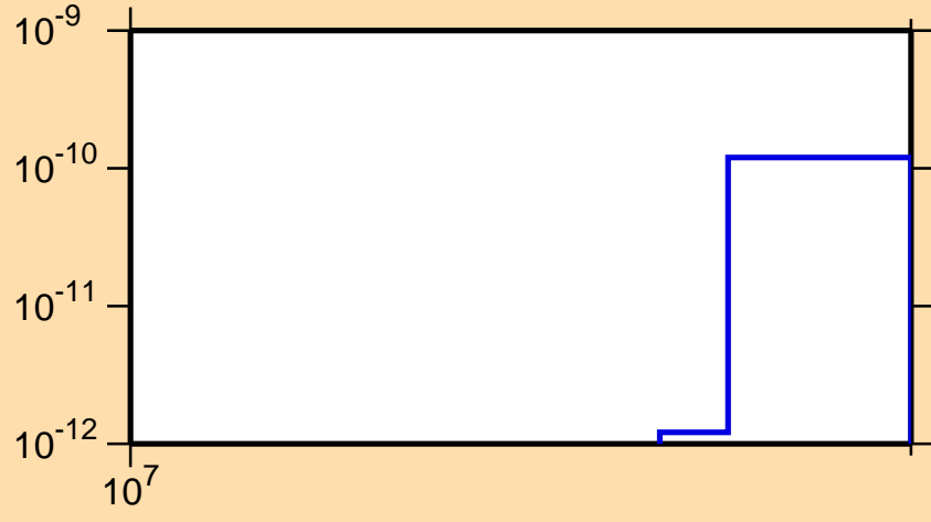
\sigma vs. E for ^{200}\text{Hg}(n,2n\alpha)
