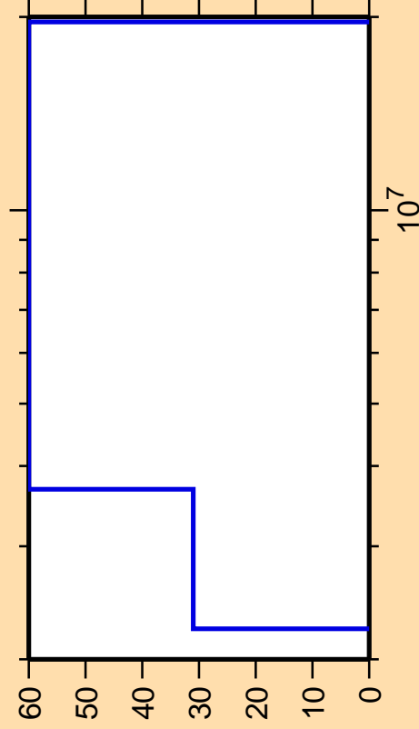
\Delta\sigma/\sigma vs. E for ^{200}\text{Hg}(n,\alpha)
