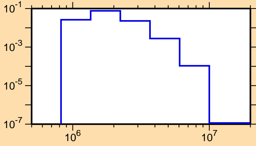
\sigma vs. E for ^{200}\text{Hg}(n,n_3)
