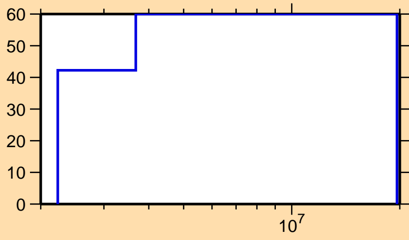
\Delta\sigma/\sigma vs. E for ^{200}\text{Hg}(n,\gamma)
