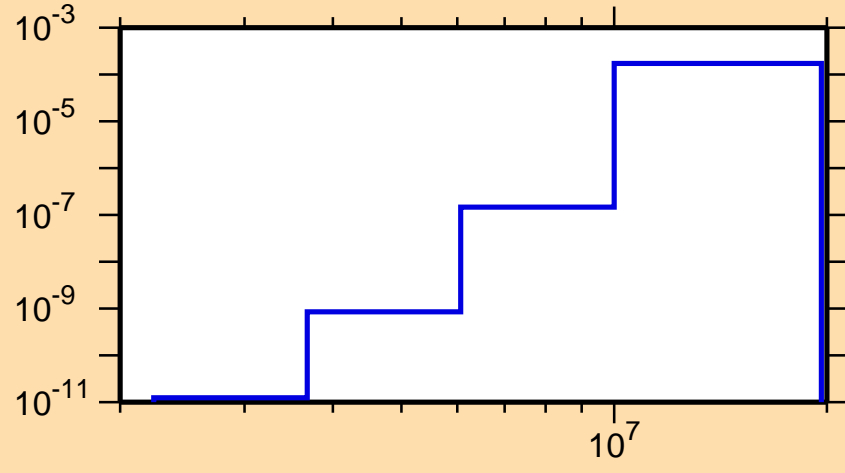
\sigma vs. E for ^{200}\text{Hg}(n,\alpha)
