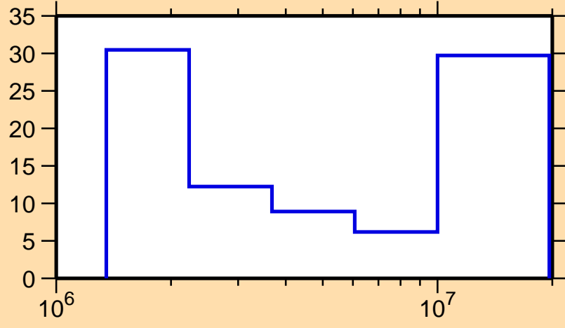
\Delta\sigma/\sigma vs. E for ^{200}\text{Hg}(n,n\text{cont.})
