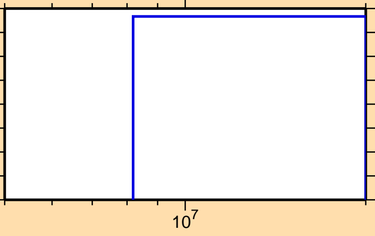
\sigma vs. E for ^{200}\text{Hg}(n,\text{He}3)
