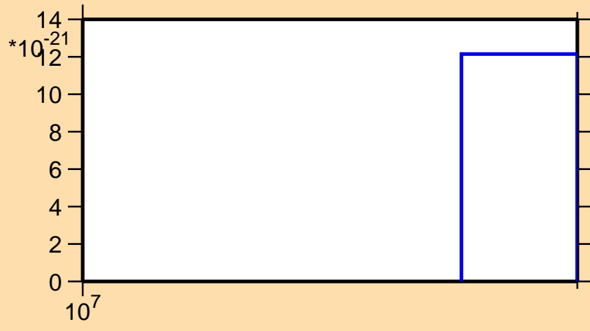
\sigma vs. E for ^{201}\text{Hg} (mt 11)
