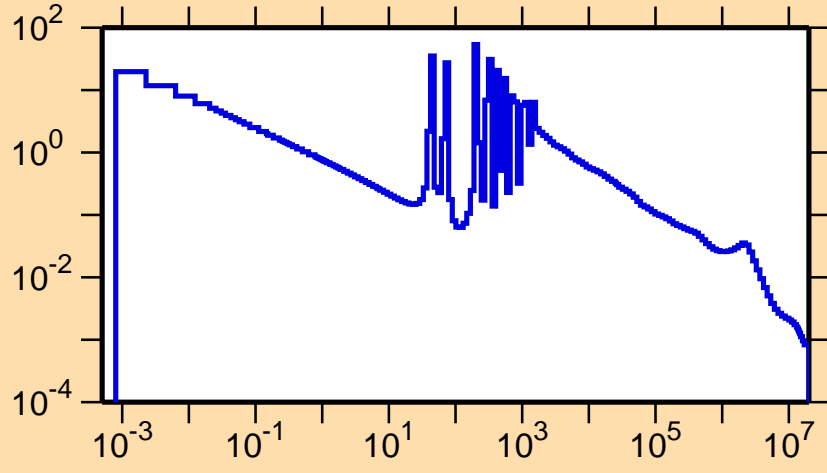
\sigma vs. E for ^{201}\text{Hg}(n,\gamma)
