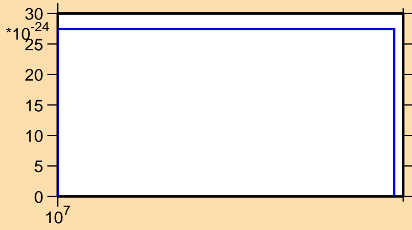
\sigma vs. E for ^{201}\text{Hg} (mt 11)
