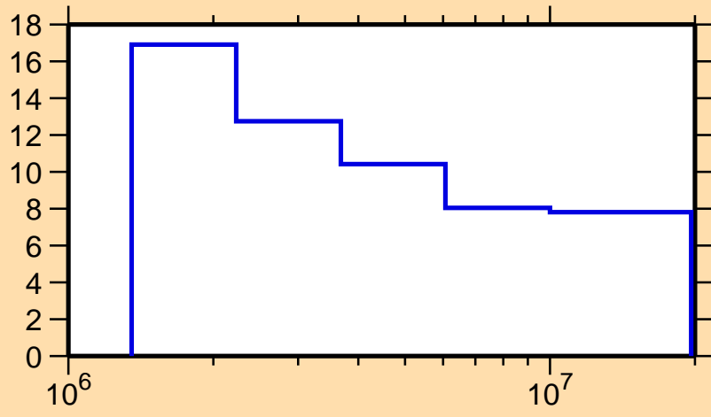
\Delta\sigma/\sigma vs. E for ^{201}\text{Hg}(n,\text{nonel.})
