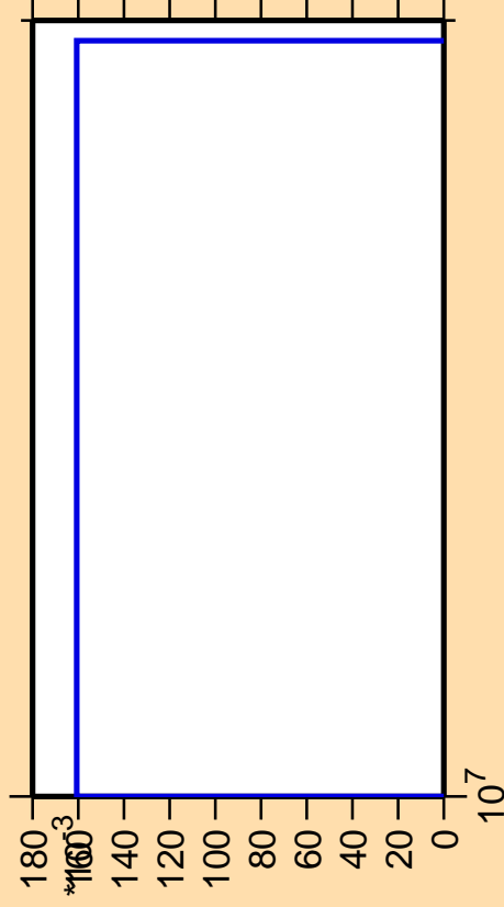
\Delta\sigma/\sigma vs. E for ^{201}\text{Hg}(n,\text{He}3)
