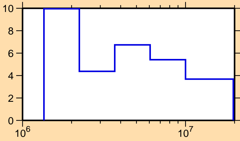
\Delta\sigma/\sigma vs. E for ^{201}\text{Hg}(n,\text{tot.})
