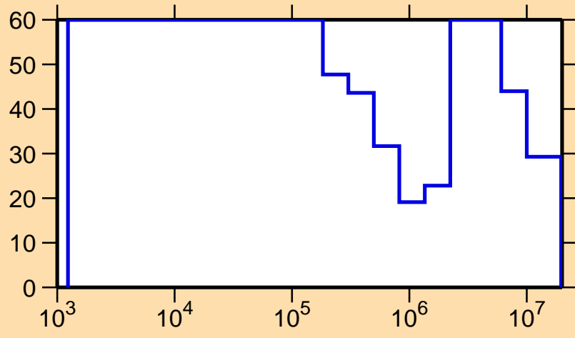
\Delta\sigma/\sigma vs. E for ^{201}\text{Hg}(n,n_1)
