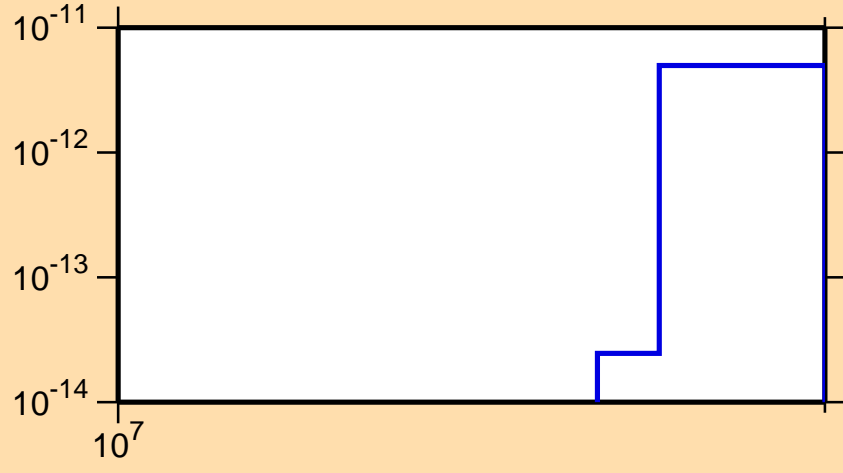
\sigma vs. E for ^{204}\text{Hg}(n,2n\alpha)
