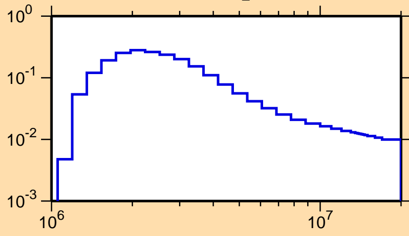
\sigma vs. E for ^{204}\text{Hg}(n,n_2)
