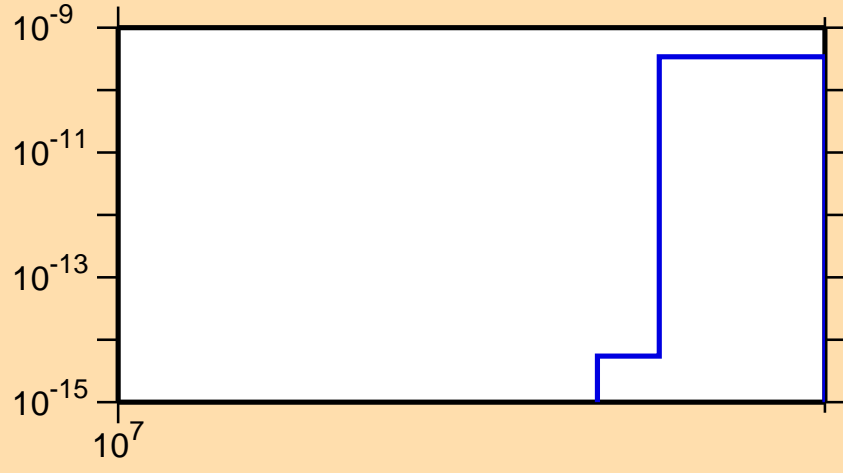
\sigma vs. E for ^{204}\text{Hg}(n,nt)
