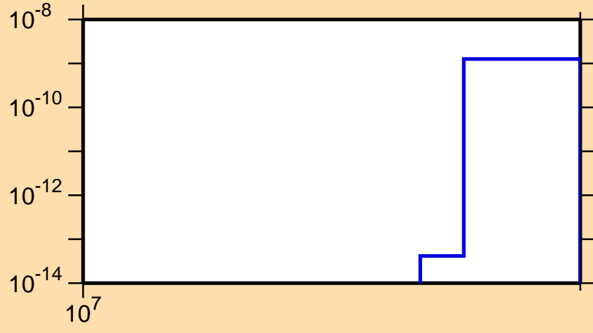
\sigma vs. E for ^{204}\text{Hg}(n,\text{nd})
