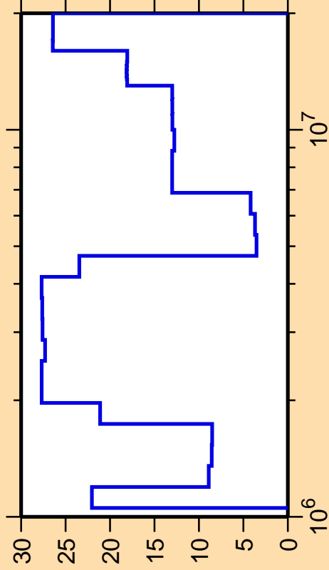
\Delta\sigma/\sigma vs. E for ^{204}\text{Hg}(n,n_2)
