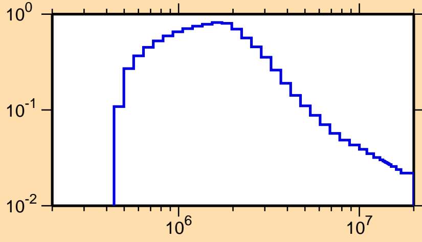
\sigma vs. E for ^{204}\text{Hg}(n,n_1)
