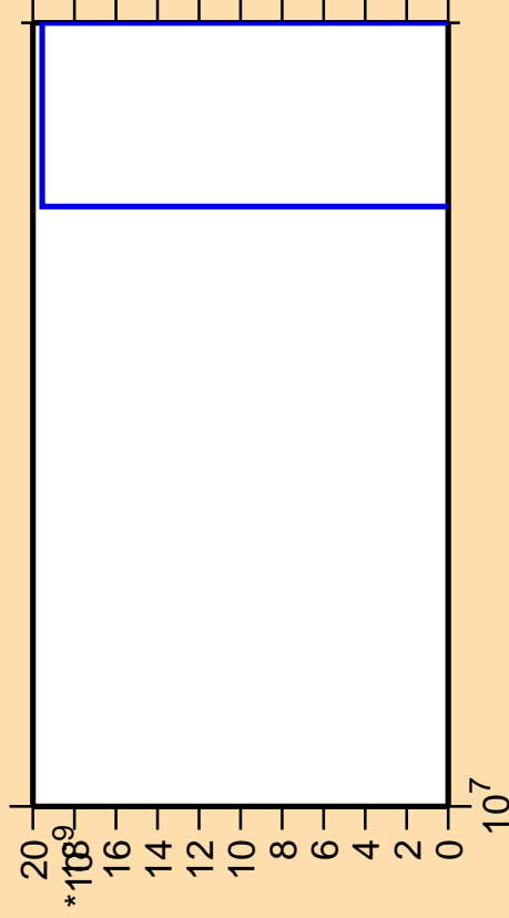
\Delta\sigma/\sigma vs. E for ^{204}\text{Hg} (mt 11)
