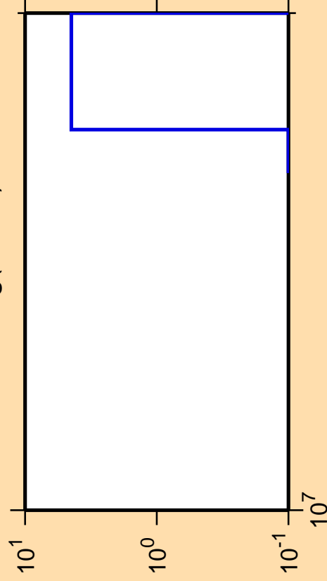
\Delta\sigma/\sigma vs. E for ^{204}\text{Hg}(n,2n\alpha)
