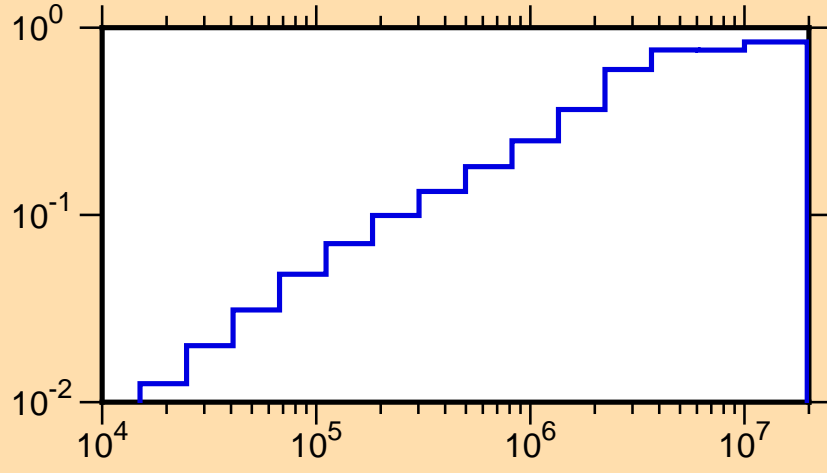
\mu vs. E for ^{204}\text{Hg}(\text{mt251})
