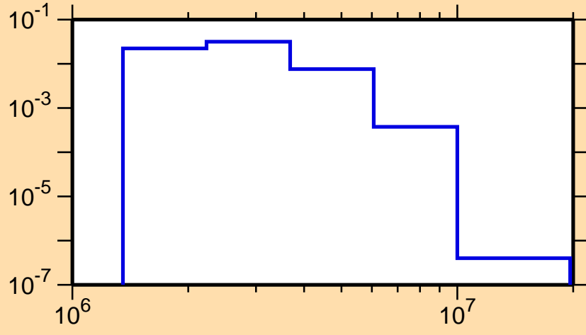
\sigma vs. E for ^{204}\text{Hg}(n,n_3)
