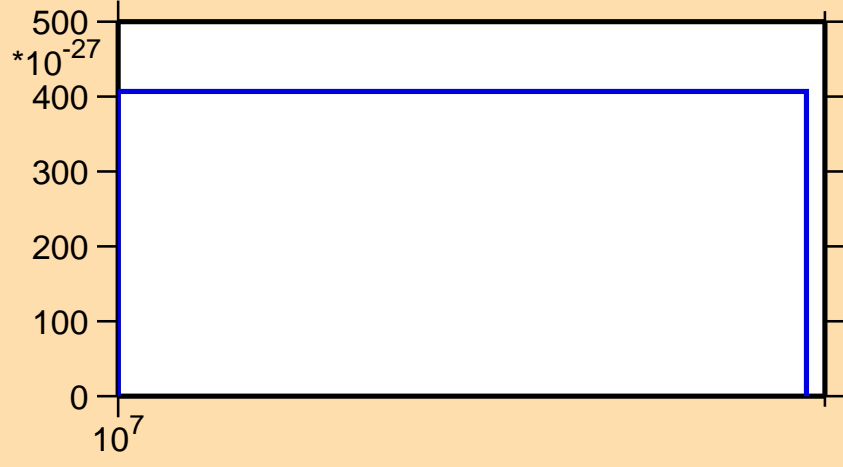
\sigma vs. E for ^{204}\text{Hg} (mt 11)
