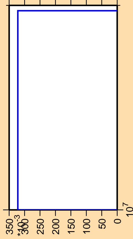
\Delta\sigma/\sigma vs. E for ^{204}\text{Hg}(n,2np)
