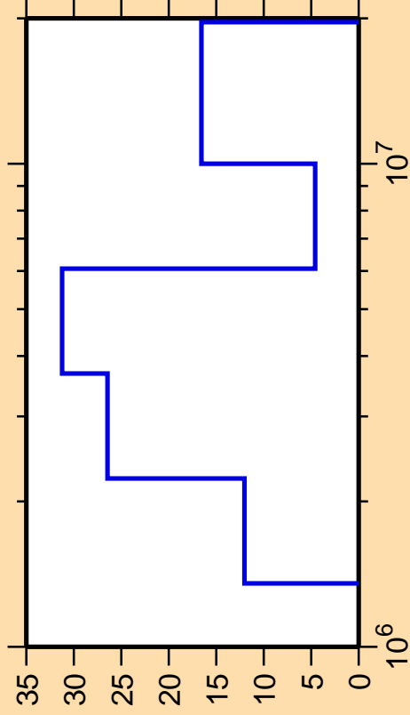
\Delta\sigma/\sigma vs. E for ^{204}\text{Hg}(n,n_4)
