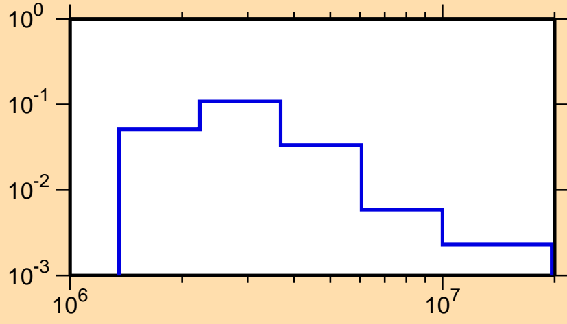
\sigma vs. E for ^{204}\text{Hg}(n,n_4)
