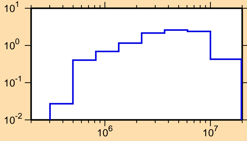
\sigma vs. E for ^{204}\text{Hg}(n,\text{inel.})
