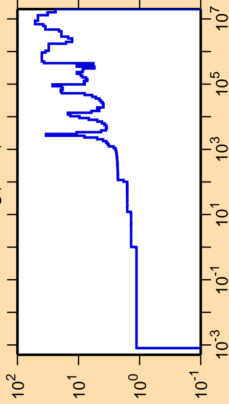
\Delta\sigma/\sigma vs. E for ^{208}\text{Hg}(n,\text{el.})
