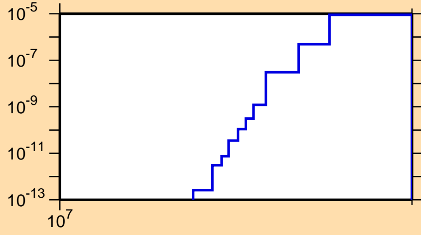
\sigma vs. E for ^{208}\text{Hg}(n,nt)
