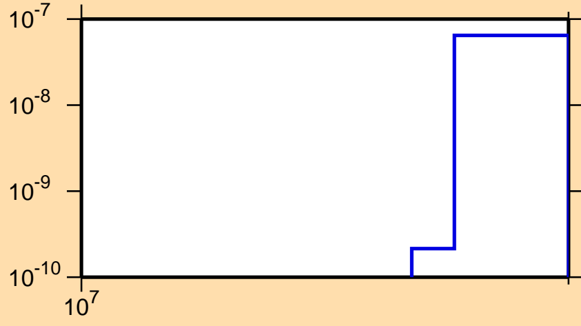
\sigma vs. E for ^{208}\text{Hg}(n,\text{nd})
