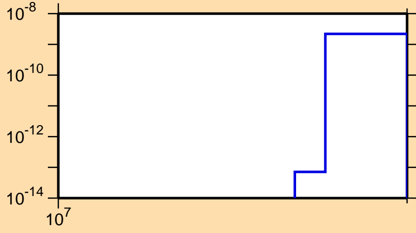
\sigma vs. E for ^{208}\text{Hg}(n,2np)
