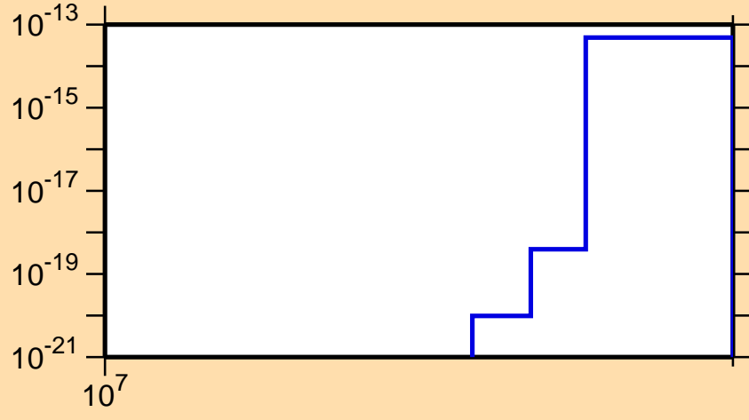
\sigma vs. E for ^{208}\text{Hg} (mt 11)
