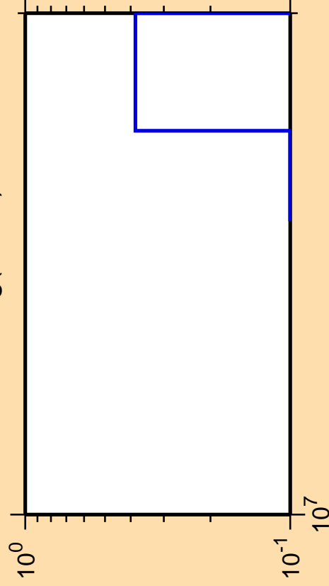
\Delta\sigma/\sigma vs. E for ^{208}\text{Hg} (mt 11)
