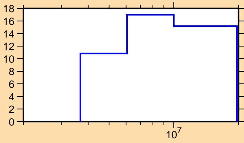
\Delta\sigma/\sigma vs. E for ^{208}\text{Hg}(n,\text{tot.})
