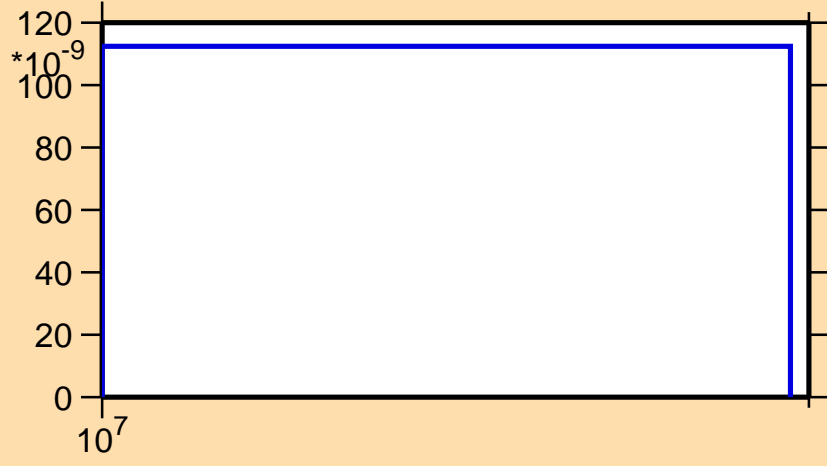
\sigma vs. E for ^{208}\text{Hg}(n,nt)
