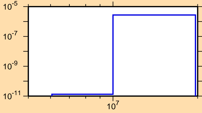
\sigma vs. E for ^{208}\text{Hg}(n,n\alpha)
