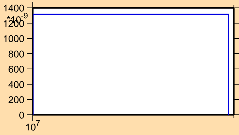
\sigma vs. E for ^{208}\text{Hg}(n,np)
