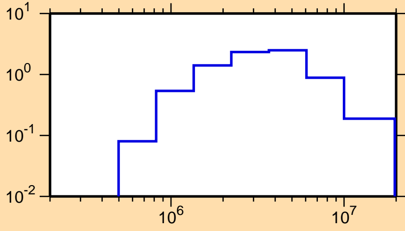
\sigma vs. E for ^{208}\text{Hg}(n,\text{inel.})
