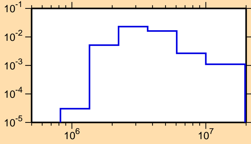
\sigma vs. E for ^{208}\text{Hg}(n,n_3)
