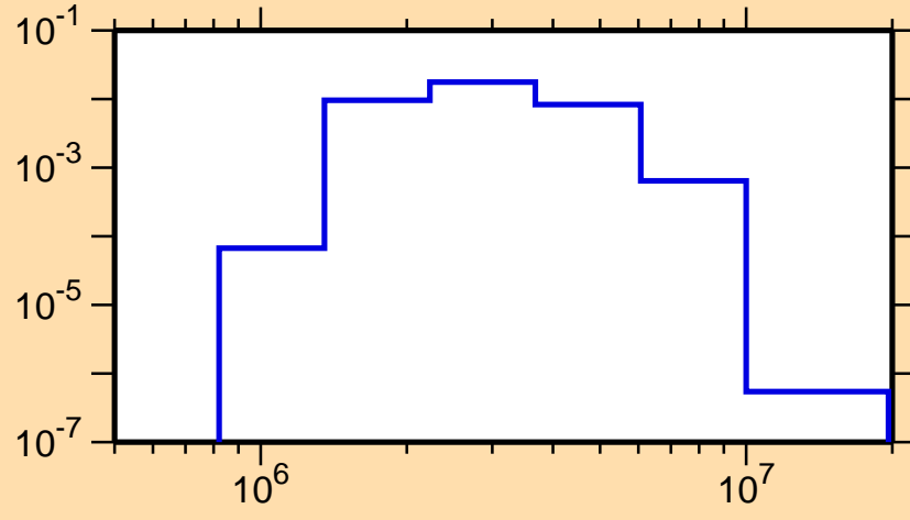
\sigma vs. E for ^{208}\text{Hg}(n,n_4)
