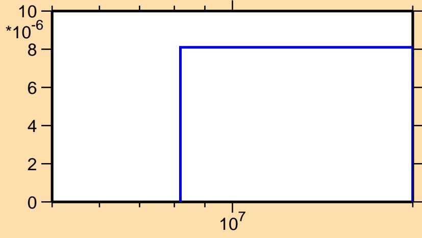
\sigma vs. E for ^{208}\text{Hg}(n,t)
