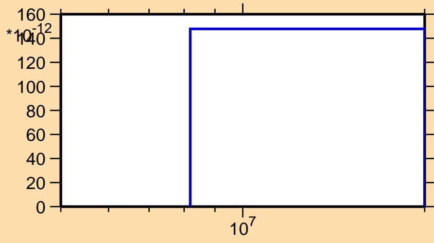
\sigma vs. E for ^{208}\text{Hg}(n,2n\alpha)
