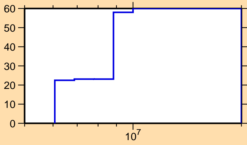
\Delta\sigma/\sigma vs. E for ^{209}\text{Hg}(n,2n)
