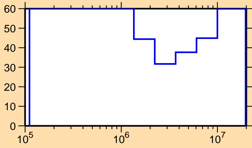
\Delta\sigma/\sigma vs. E for ^{209}\text{Hg}(n,n\text{cont.})
