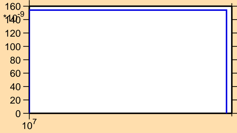
\sigma vs. E for ^{209}\text{Hg}(n,nt)
