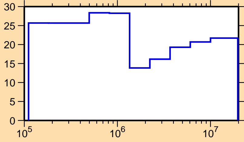
\Delta\sigma/\sigma vs. E for ^{209}\text{Hg}(n, el.)
