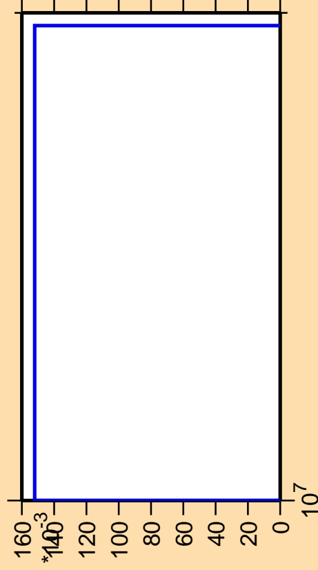
\Delta\sigma/\sigma vs. E for ^{209}\text{Hg}(n,3n\alpha)
