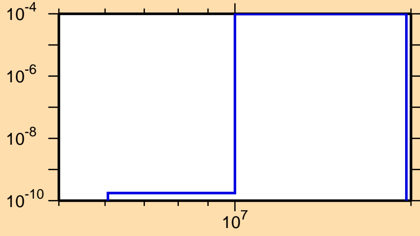
\sigma vs. E for ^{209}\text{Hg}(n,p)
