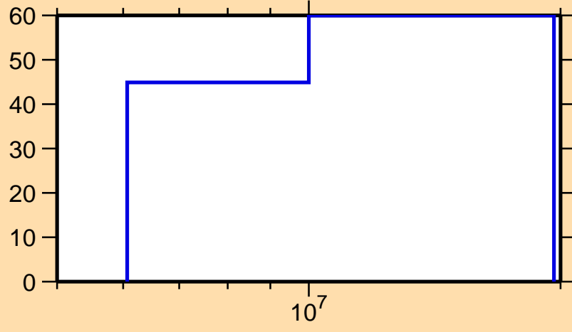
\Delta\sigma/\sigma vs. E for ^{209}\text{Hg}(n,ncont.)
