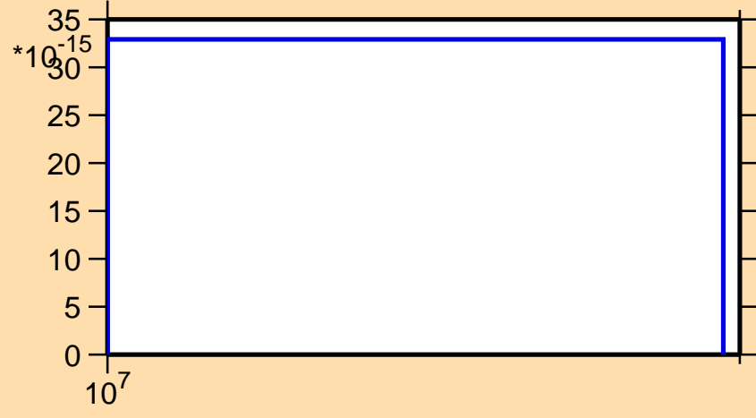
\sigma vs. E for ^{209}\text{Hg}(n,3n\alpha)
