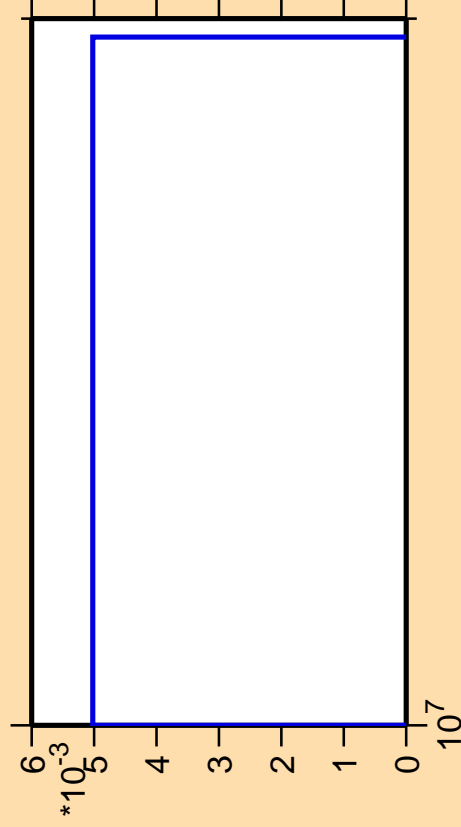
\Delta\sigma/\sigma vs. E for ^{209}\text{Hg} (mt 11)
