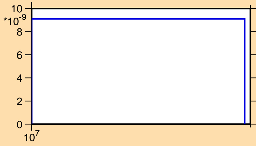
\sigma vs. E for ^{209}\text{Hg}(n,\text{nd})
