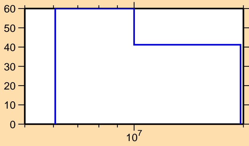
\Delta\sigma/\sigma vs. E for ^{209}\text{Hg}(n,\gamma)
