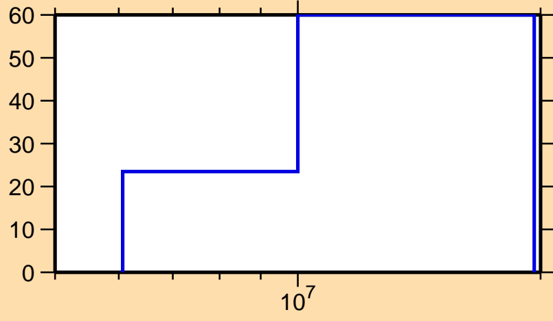
\Delta\sigma/\sigma vs. E for ^{209}\text{Hg}(n,2n)
