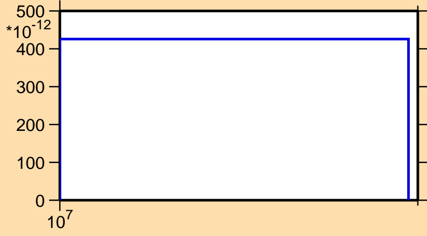
\sigma vs. E for ^{209}\text{Hg}(n,2np)
