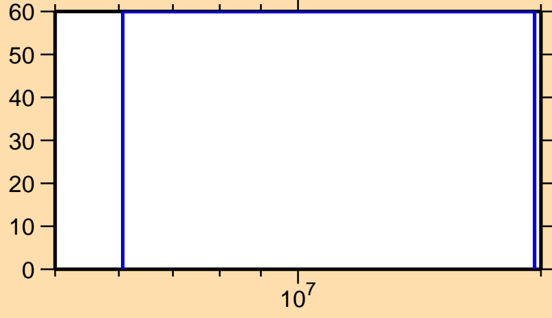
\Delta\sigma/\sigma vs. E for ^{209}\text{Hg}(n,n_1)
