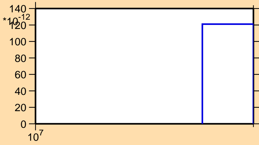
\sigma vs. E for ^{211}\text{Hg}(n,3n\alpha)
