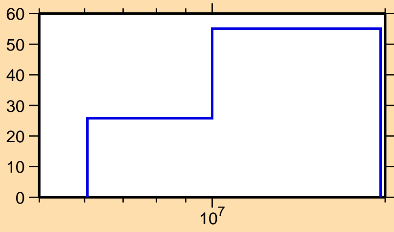
\Delta\sigma/\sigma vs. E for ^{211}\text{Hg}(n,p)
