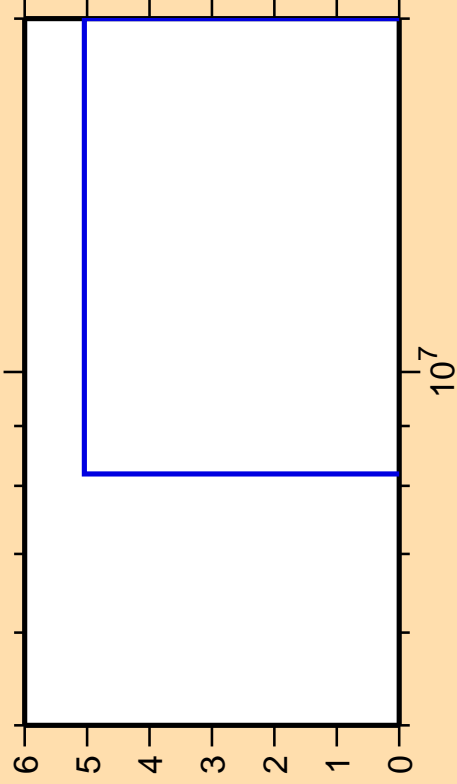
\Delta\sigma/\sigma vs. E for ^{211}\text{Hg}(n,3n\alpha)
