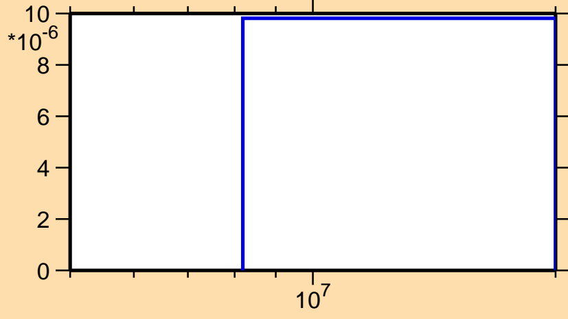
\sigma vs. E for ^{211}\text{Hg}(n,t)
