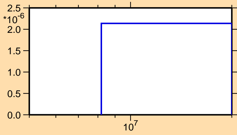
\sigma vs. E for ^{211}\text{Hg}(n,d)
