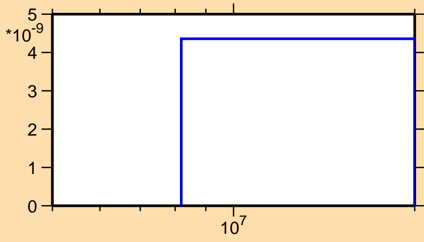
\sigma vs. E for ^{211}\text{Hg}(n,\text{nd})
