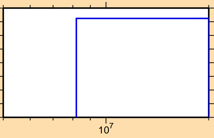
\sigma vs. E for ^{211}\text{Hg}(n,2n\alpha)
