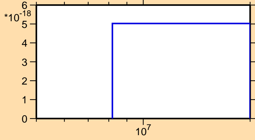
\sigma vs. E for ^{211}\text{Hg} (mt 42)
