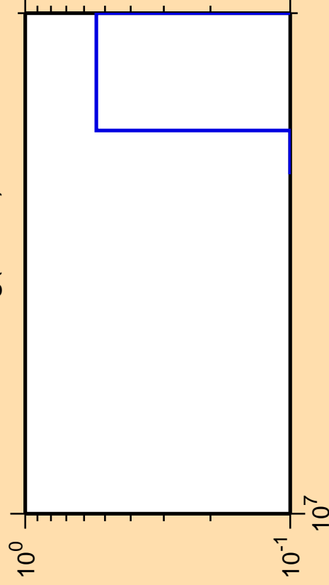
\Delta\sigma/\sigma vs. E for ^{212}\text{Hg} (mt 11)
