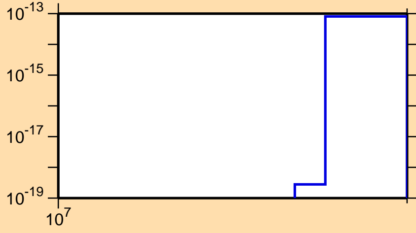
\sigma vs. E for ^{212}\text{Hg} (mt 11)
