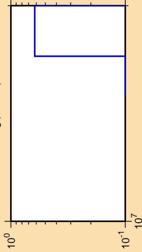
\Delta\sigma/\sigma vs. E for ^{214}\text{Hg} (mt 11)
