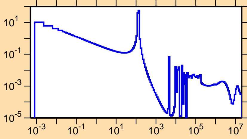
\sigma vs. E for ^{214}\text{Hg}(n,\gamma)
