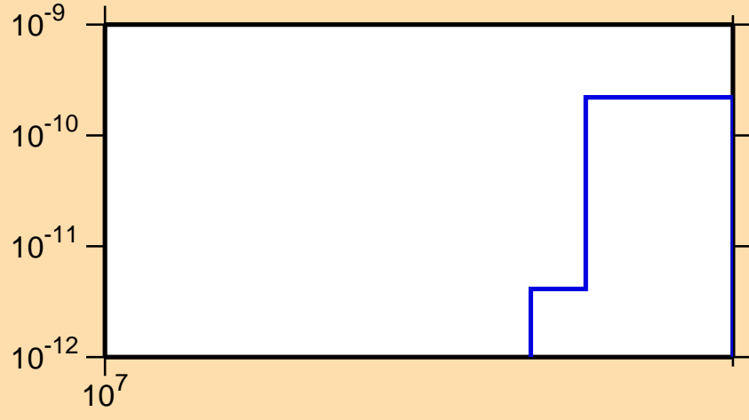
\sigma vs. E for ^{214}\text{Hg}(n,3n\alpha)
