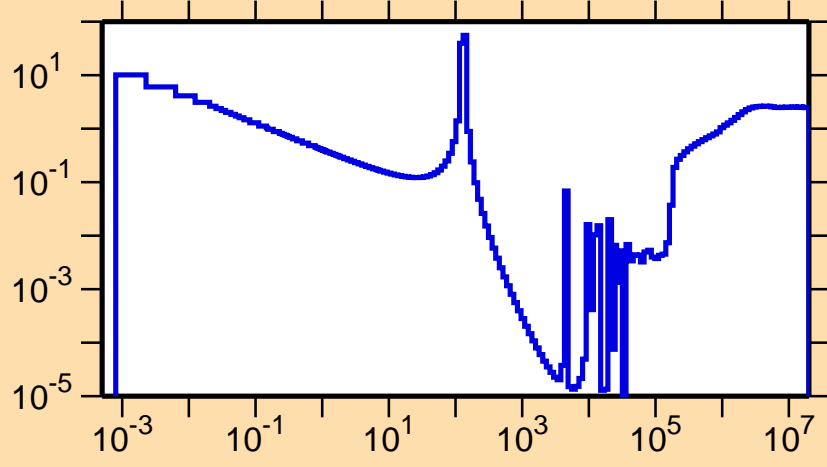
\sigma vs. E for ^{214}\text{Hg}(n,\text{nonel.})
