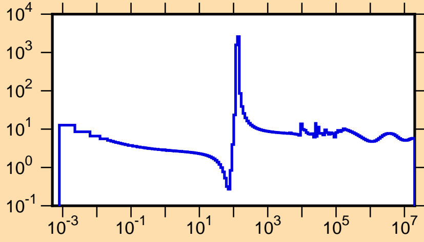
\sigma vs. E for ^{214}\text{Hg}(n,\text{tot.})
