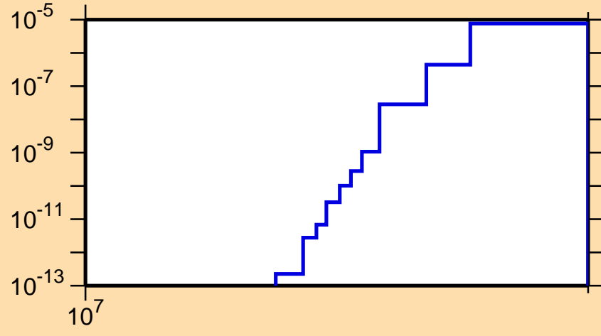
\sigma vs. E for ^{214}\text{Hg}(n,nt)
