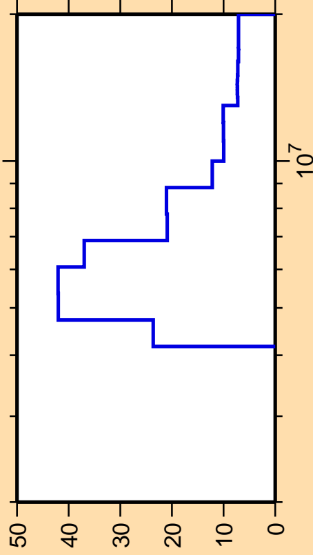
\Delta\sigma/\sigma vs. E for ^{214}\text{Hg}(n,n\text{cont.})
