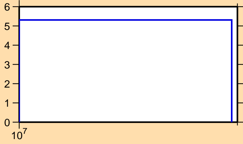
\Delta\sigma/\sigma vs. E for ^{214}\text{Hg}(n,\text{nonel.})
