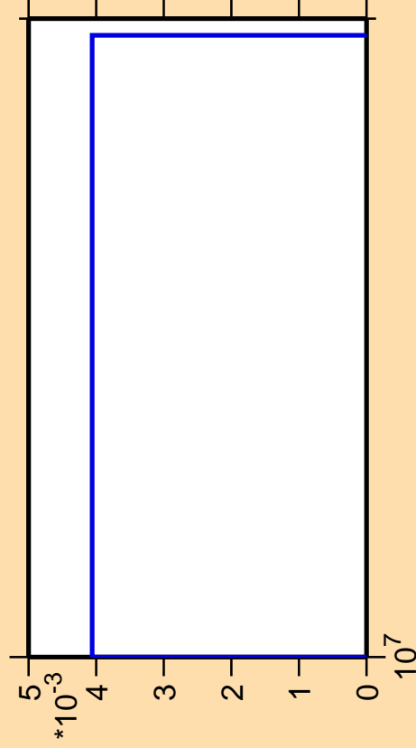
\Delta\sigma/\sigma vs. E for ^{214}\text{Hg} (mt 11)
