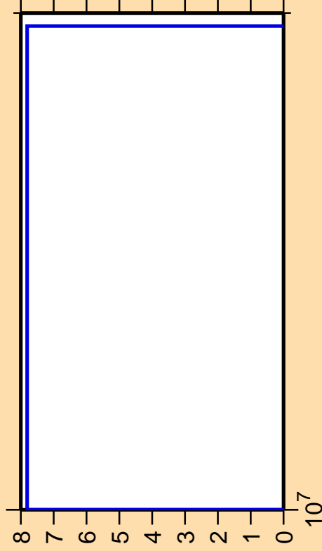
\Delta\sigma/\sigma vs. E for ^{214}\text{Hg}(n,3n\alpha)
