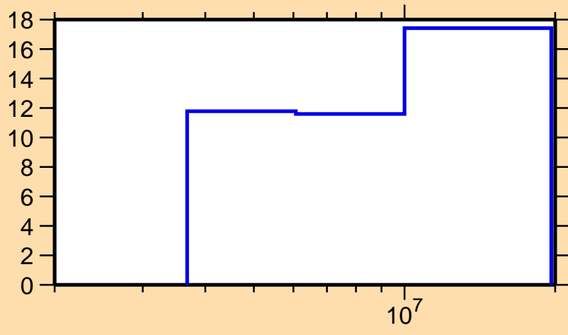
\Delta\sigma/\sigma vs. E for ^{214}\text{Hg}(n,2n)
