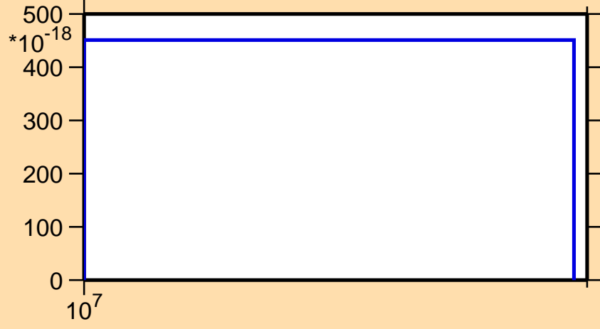
\sigma vs. E for ^{214}\text{Hg} (mt 11)
