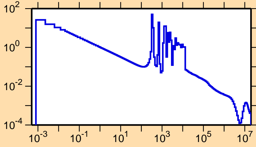
\sigma vs. E for ^{215}\text{Hg}(n,\gamma)
