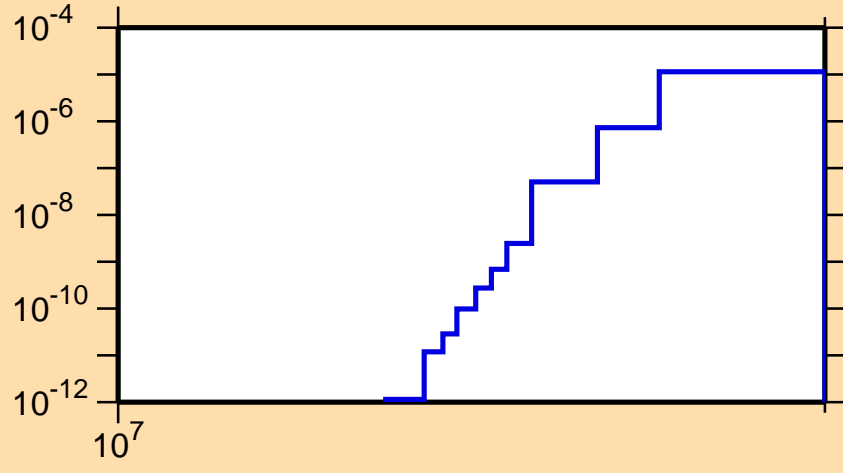
\sigma vs. E for ^{215}\text{Hg}(n,nt)
