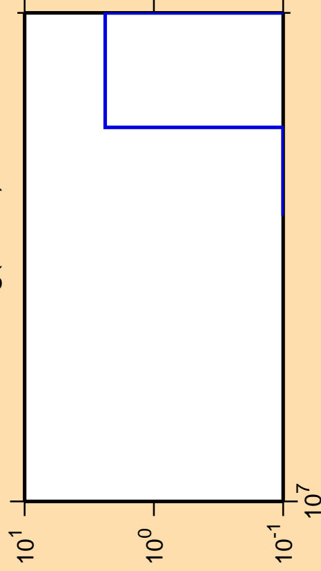
\Delta\sigma/\sigma vs. E for ^{215}\text{Hg} (mt 11)
