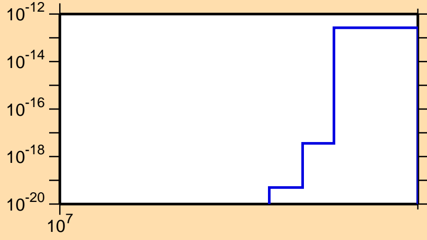
\sigma vs. E for ^{215}\text{Hg} (mt 11)
