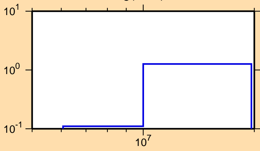
\sigma vs. E for ^{215}\text{Hg}(n,3n)
