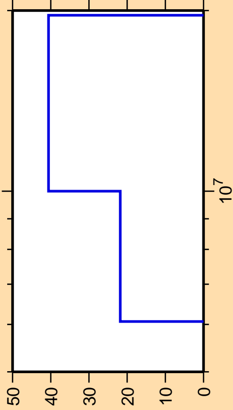
\Delta\sigma/\sigma vs. E for ^{215}\text{Hg}(n,3n)
