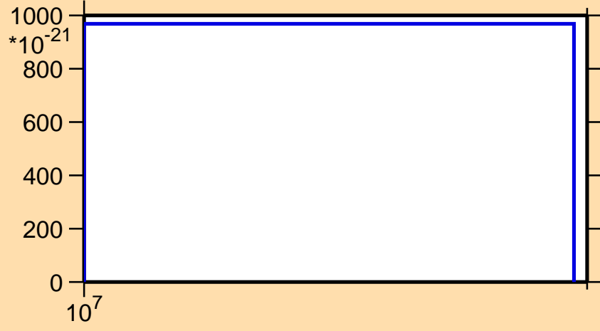
\sigma vs. E for ^{215}\text{Hg} (mt 42)
