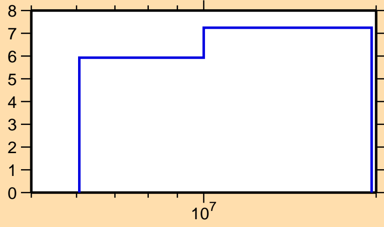
\Delta\sigma/\sigma vs. E for ^{215}\text{Hg}(n,\text{nonel.})
