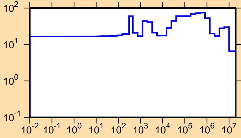
\Delta\sigma/\sigma vs. E for ^{215}\text{Hg}(n,\text{el.})
