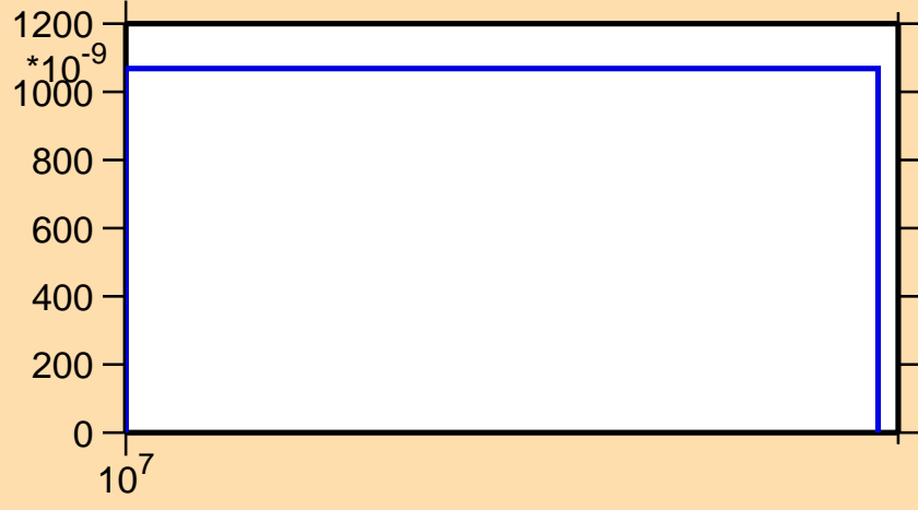
\sigma vs. E for ^{215}\text{Hg}(n,d)
