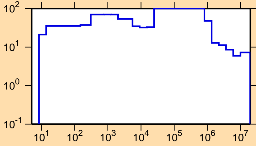
\Delta\sigma/\sigma vs. E for ^{215}\text{Hg}(n,\text{nonel.})
