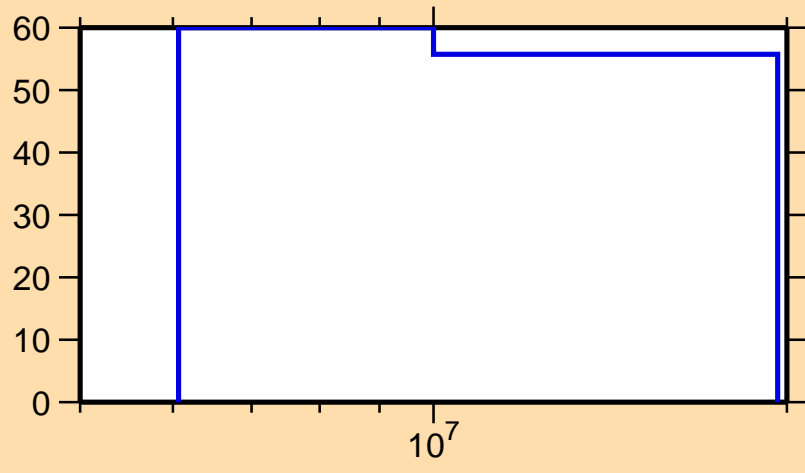
\Delta\sigma/\sigma vs. E for ^{215}\text{Hg}(n,n_1)
