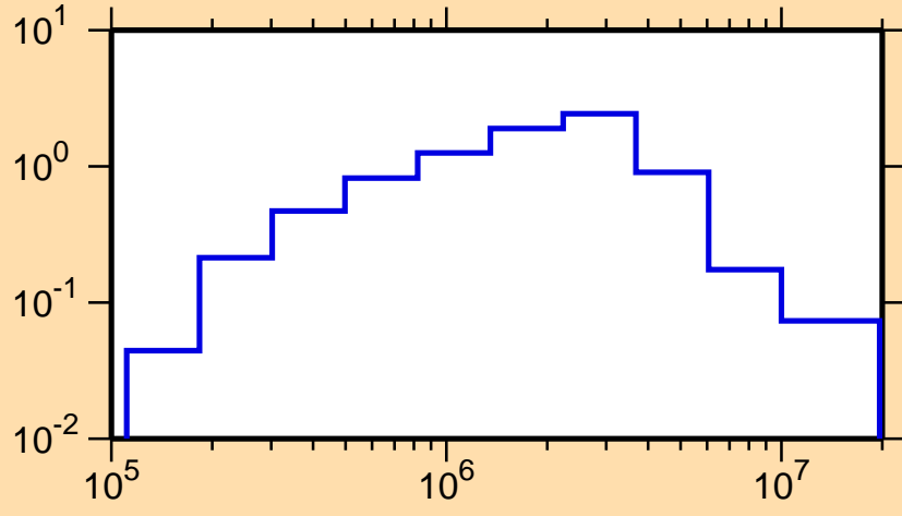
\sigma vs. E for ^{215}\text{Hg}(n,\text{inel.})
