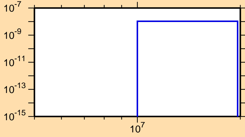
\sigma vs. E for ^{215}\text{Hg}(n,2n\alpha)
