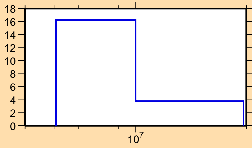
\Delta\sigma/\sigma vs. E for ^{215}\text{Hg}(n,\text{tot.})
