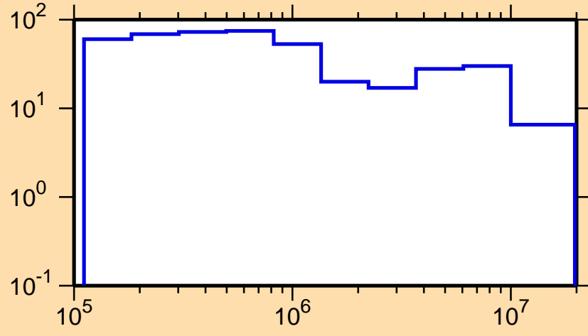
\Delta\sigma/\sigma vs. E for ^{215}\text{Hg}(n, el.)
