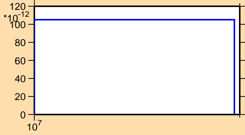
\sigma vs. E for ^{215}\text{Hg}(n,2np)
