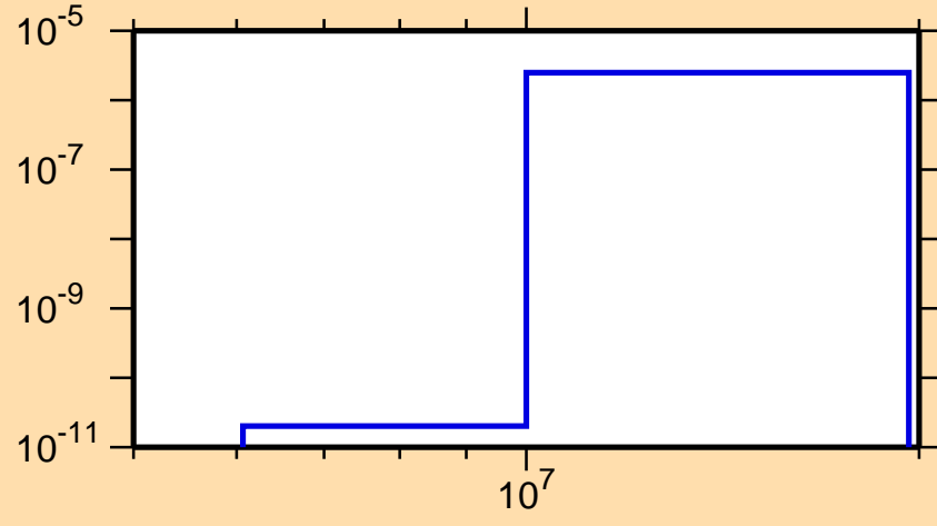
\sigma vs. E for ^{215}\text{Hg}(n,\alpha)
