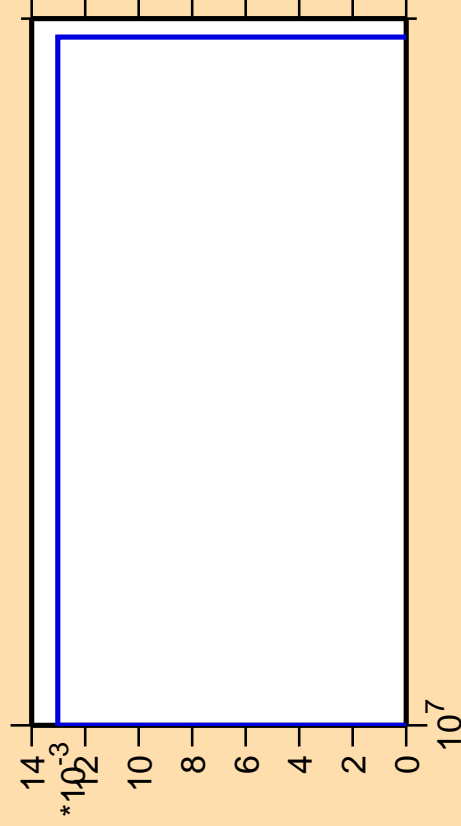
\Delta\sigma/\sigma vs. E for ^{215}\text{Hg} (mt 11)
