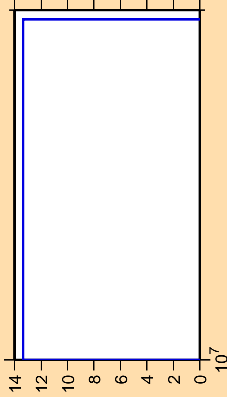
\Delta\sigma/\sigma vs. E for ^{215}\text{Hg}(n,3n\alpha)
