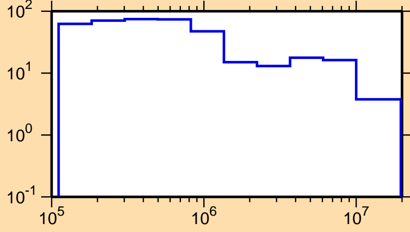
\Delta\sigma/\sigma vs. E for ^{215}\text{Hg}(n,\text{tot.})
