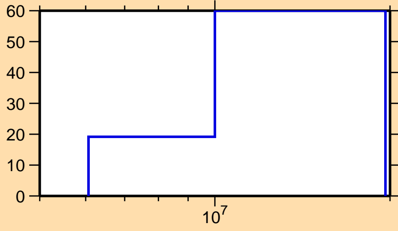
\Delta\sigma/\sigma vs. E for ^{215}\text{Hg}(n,2n)
