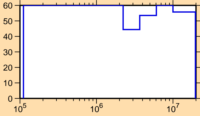
\Delta\sigma/\sigma vs. E for ^{215}\text{Hg}(n,n_1)
