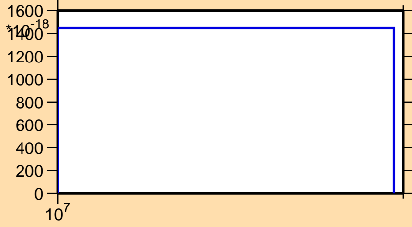
\sigma vs. E for ^{215}\text{Hg} (mt 11)
