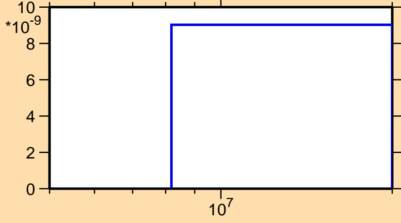
\sigma vs. E for ^{215}\text{Hg}(n,2n\alpha)
