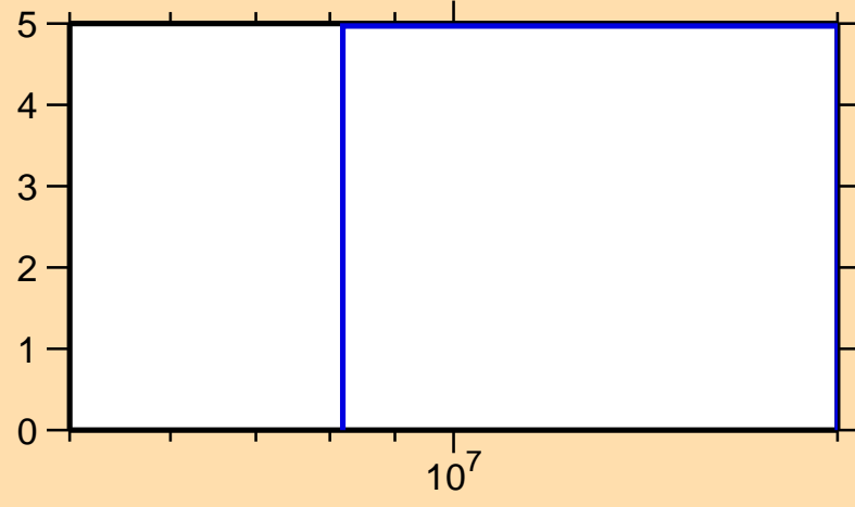
\Delta\sigma/\sigma vs. E for ^{215}\text{Hg}(n,\text{tot.})
