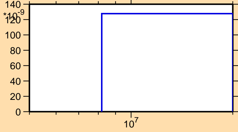
\sigma vs. E for ^{215}\text{Hg}(n,nt)
