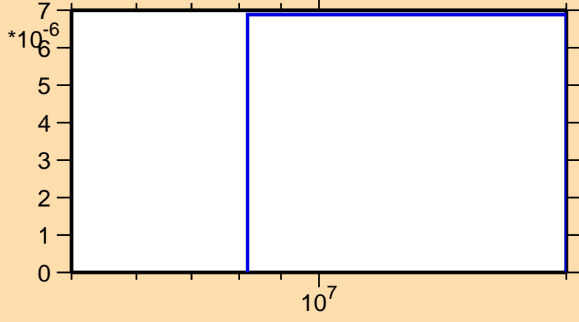
\sigma vs. E for ^{215}\text{Hg}(n,t)
