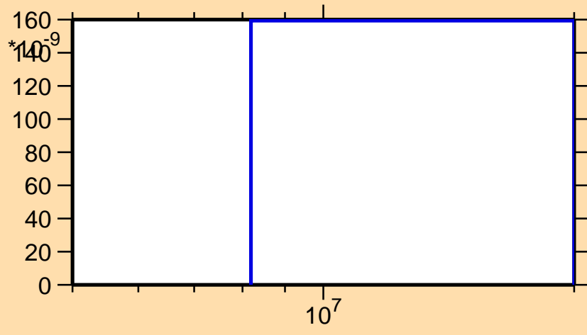
\sigma vs. E for ^{215}\text{Hg}(n,np)
