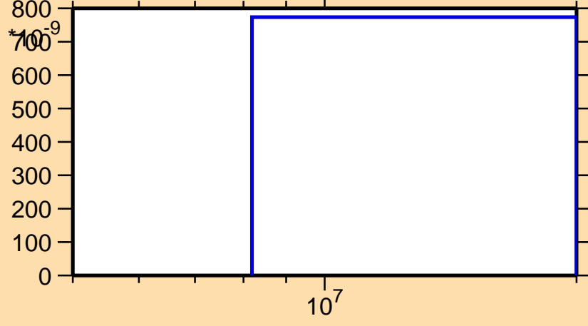
\sigma vs. E for ^{215}\text{Hg}(n,n\alpha)
