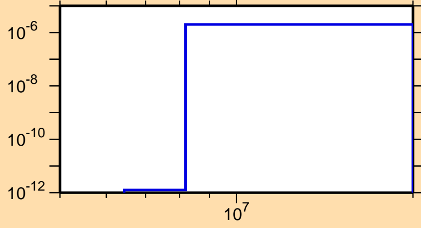
\sigma vs. E for ^{215}\text{Hg}(n,\alpha)
