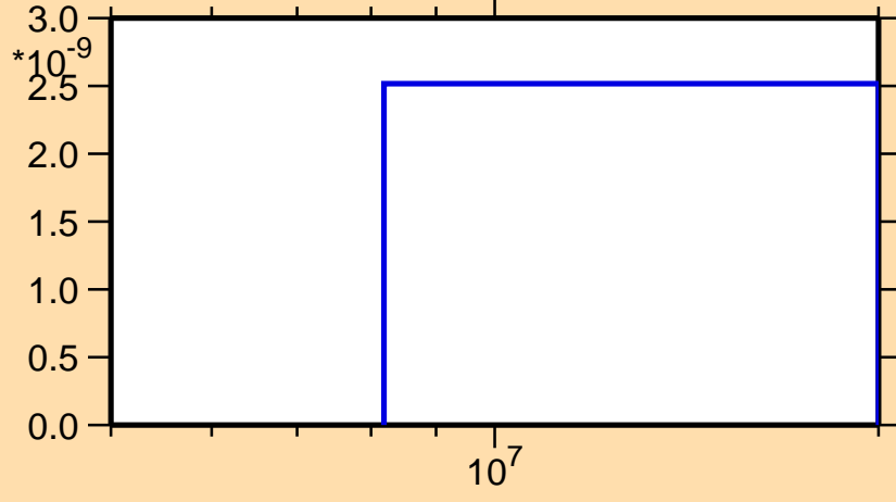
\sigma vs. E for ^{215}\text{Hg}(n,\text{nd})
