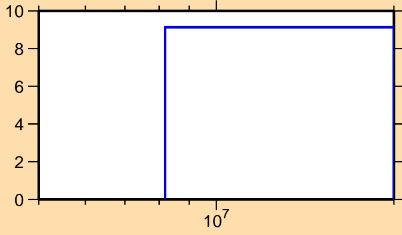
\Delta\sigma/\sigma vs. E for ^{215}\text{Hg}(n,\text{el.})
