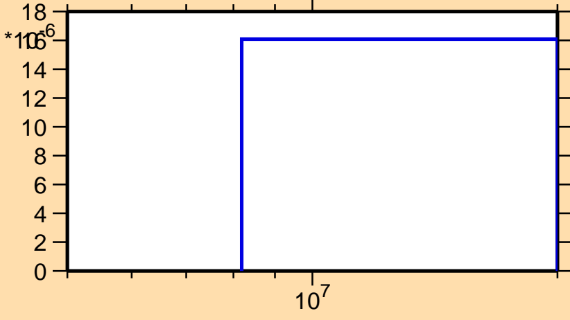
\sigma vs. E for ^{215}\text{Hg}(n,p)
