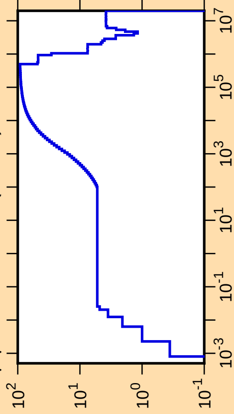
\Delta\mu/\mu vs. E for ^{145}\text{Ho}(\text{mt251})
