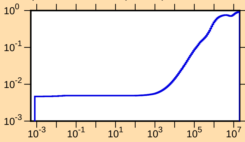
\mu vs. E for ^{145}\text{Ho}(\text{mt251})
