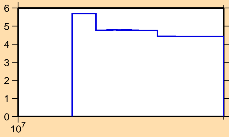
\Delta\sigma/\sigma vs. E for ^{145}\text{Ho}(n,\text{el.})
