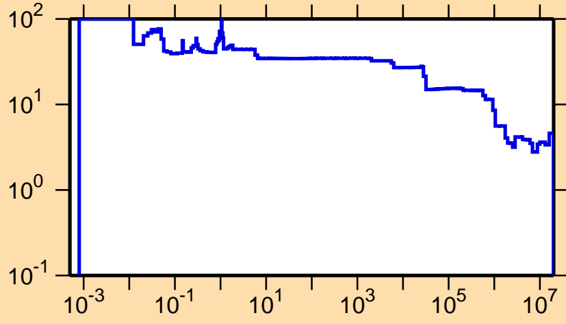
\Delta\sigma/\sigma vs. E for ^{145}\text{Ho}(n,\text{nonel.})
