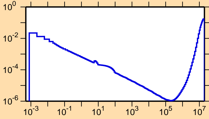
\sigma vs. E for ^{145}\text{Ho}(n,p\alpha)
