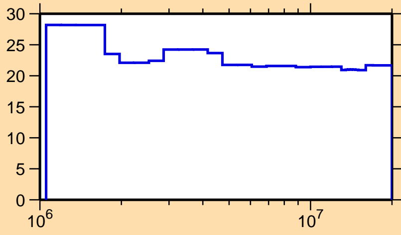
\Delta\sigma/\sigma vs. E for ^{145}\text{Ho}(n,n_1)
