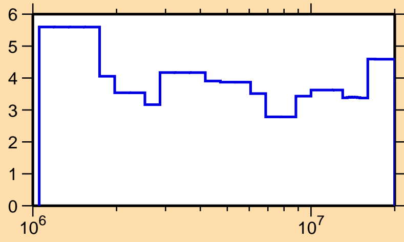
\Delta\sigma/\sigma vs. E for ^{145}\text{Ho}(n,\text{nonel.})
