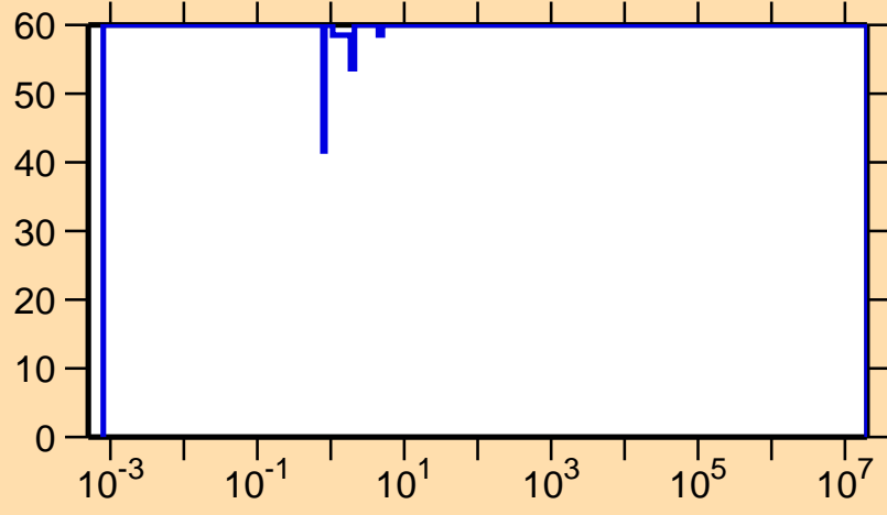
\Delta\sigma/\sigma vs. E for ^{145}\text{Ho}(n,\gamma)
