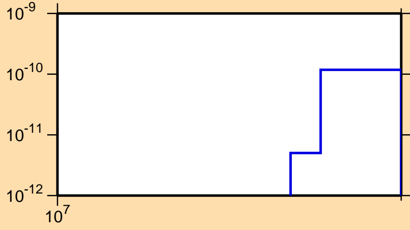
\sigma vs. E for ^{145}\text{Ho}(n,2n\alpha)
