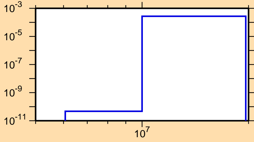
\sigma vs. E for ^{145}\text{Ho}(n,t)
