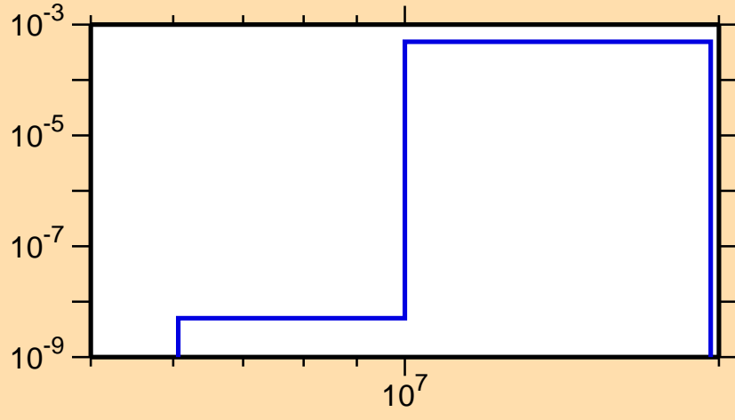
\sigma vs. E for ^{145}\text{Ho}(n,\text{pd})
