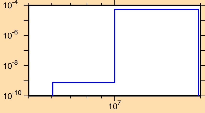
\sigma vs. E for ^{145}\text{Ho} (mt 45)
