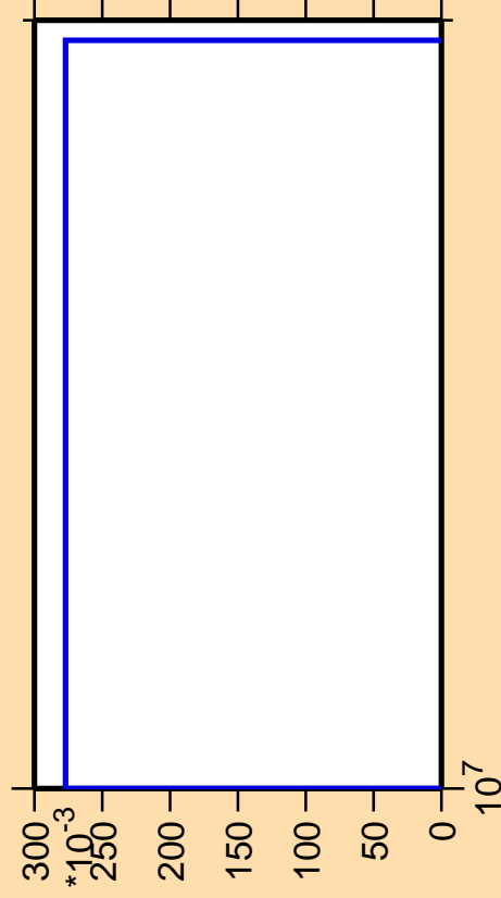
\Delta\sigma/\sigma vs. E for ^{145}\text{Ho}(n,nt)
