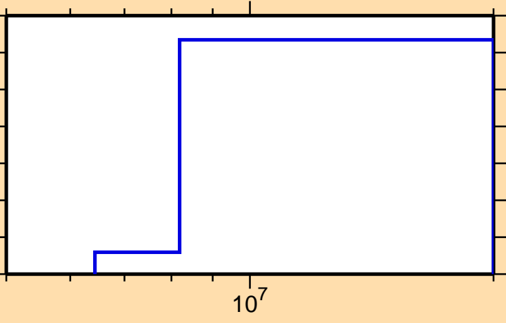
\sigma vs. E for ^{145}\text{Ho}(\text{mt117})
