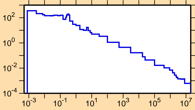
\sigma vs. E for ^{145}\text{Ho}(n,\gamma)
