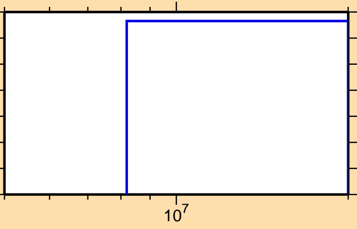
\sigma vs. E for ^{145}\text{Ho}(n,2np)
