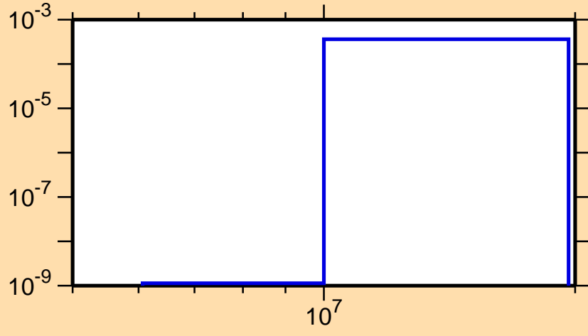
\sigma vs. E for ^{146}\text{Ho}(n,\text{pd})
