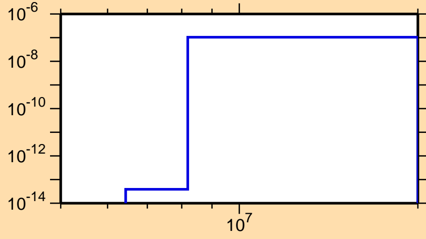
\sigma vs. E for ^{146}\text{Ho}(\text{mt117})
