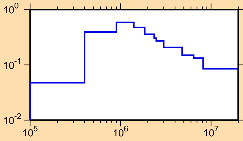
\sigma vs. E for ^{146}\text{Ho}(n,n_1)
