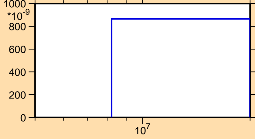
\sigma vs. E for ^{146}\text{Ho}(n,\text{nd})
