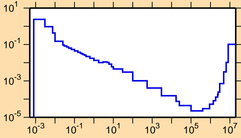
\sigma vs. E for ^{146}\text{Ho}(n,p\alpha)
