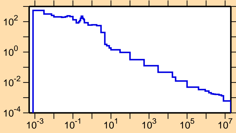
\sigma vs. E for ^{146}\text{Ho}(n,\gamma)
