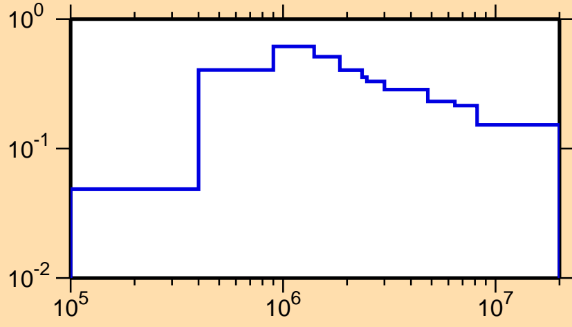
\sigma vs. E for ^{146}\text{Ho}(n,\text{inel.})
