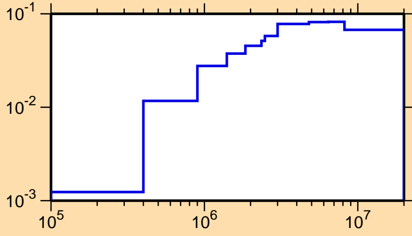
\sigma vs. E for ^{146}\text{Ho}(n,n\text{cont.})
