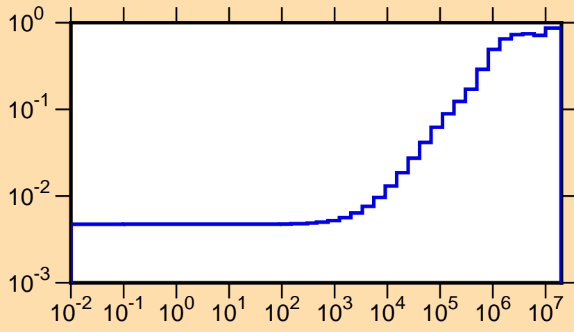
\mu vs. E for ^{148}\text{Ho}(\text{mt251})
