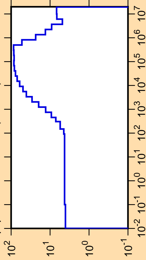
\Delta\mu/\mu vs. E for ^{148}\text{Ho}(\text{mt251})
