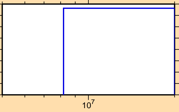
\sigma vs. E for ^{148}\text{Ho}(\text{mt } 45)
