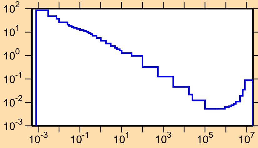
\sigma vs. E for ^{148}\text{Ho}(n,\alpha)
