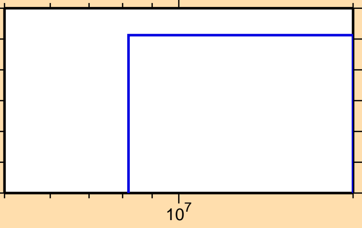
\sigma vs. E for ^{148}\text{Ho}(\text{mt117})
