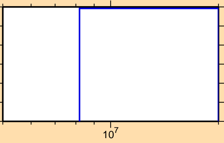
\sigma vs. E for ^{148}\text{Ho}(n,\text{pd})
