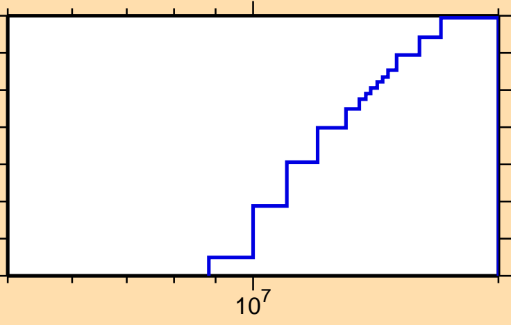
\sigma vs. E for ^{148}\text{Ho}(\text{mt117})
