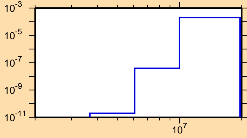
\sigma vs. E for ^{148}\text{Ho}(n,\text{He3})
