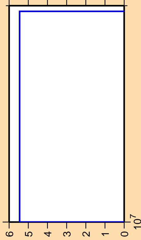
\Delta\sigma/\sigma vs. E for ^{149}\text{Ho}(n,nt)
