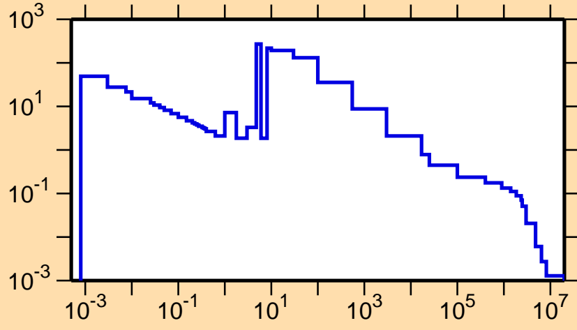
\sigma vs. E for ^{149}\text{Ho}(n,\gamma)
