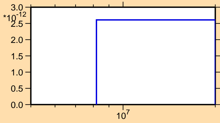
\sigma vs. E for ^{149}\text{Ho} (mt 34)
