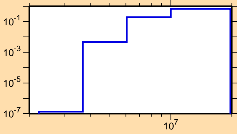
\sigma vs. E for ^{150}\text{Ho}(n,np)
