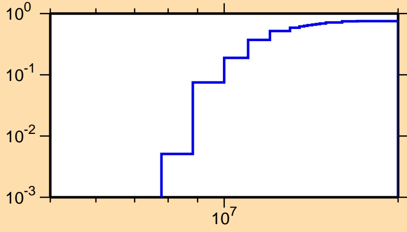
\sigma vs. E for ^{150}\text{Ho}(n,2n)
