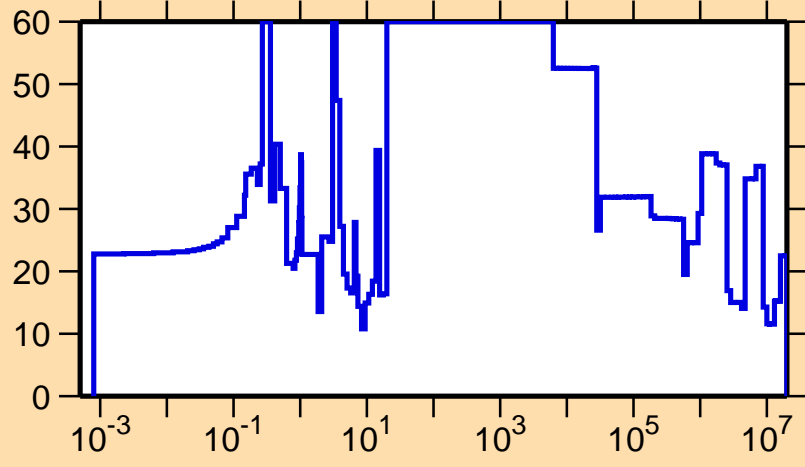
\Delta\sigma/\sigma vs. E for ^{150}\text{Ho}(n,\text{el.})
