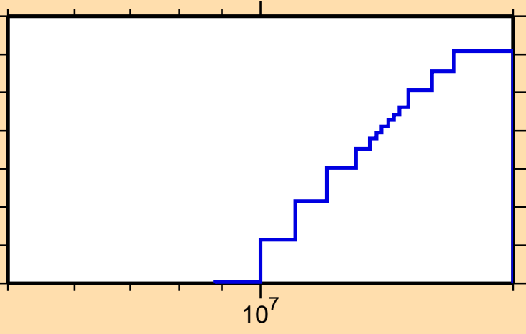
\sigma vs. E for ^{150}\text{Ho}(\text{mt117})
