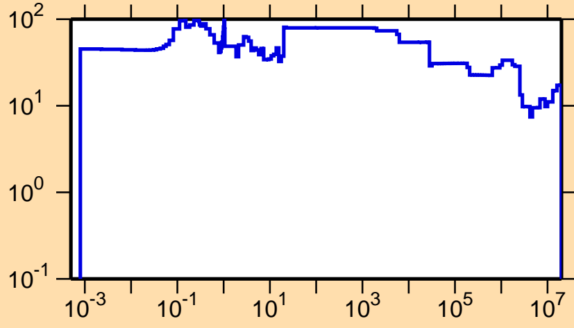
\Delta\sigma/\sigma vs. E for ^{150}\text{Ho}(n,\text{tot.})
