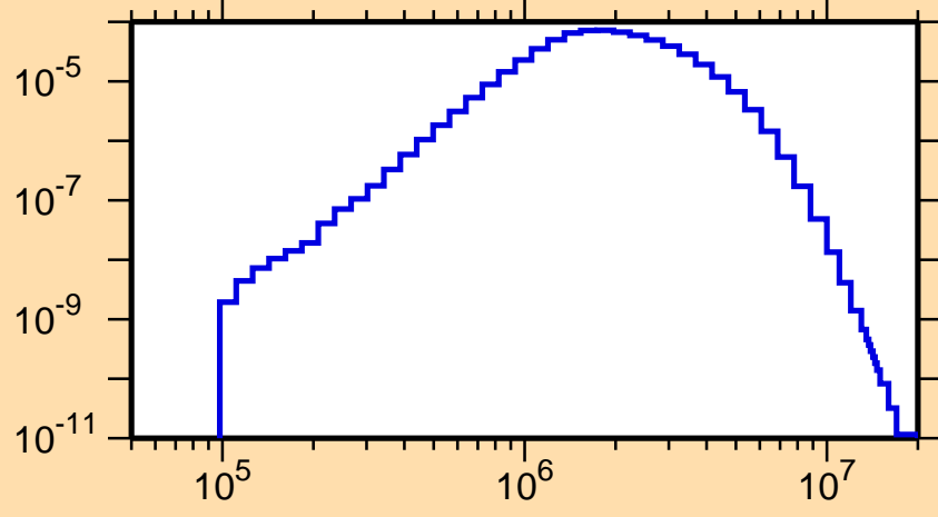
\sigma vs. E for ^{150}\text{Ho}(n,n_1)
