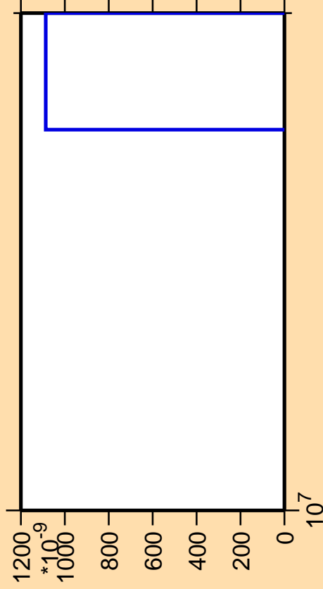
\Delta\sigma/\sigma vs. E for ^{150}\text{Ho} (mt 11)
