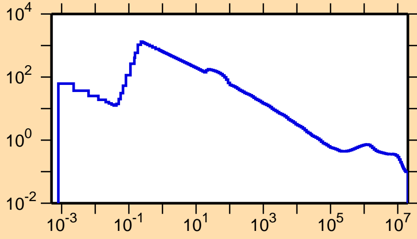
\sigma vs. E for ^{150}\text{Ho}(n,p)
