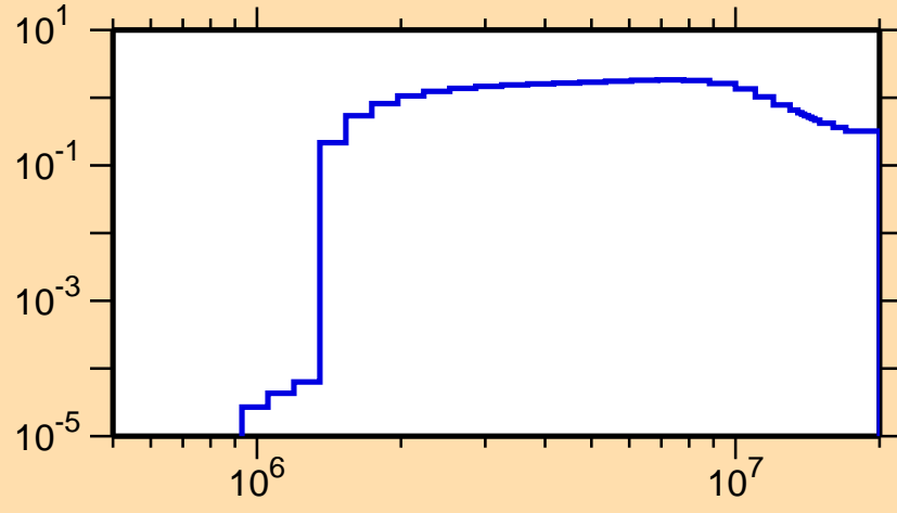
\sigma vs. E for ^{150}\text{Ho}(n,\text{inel.})
