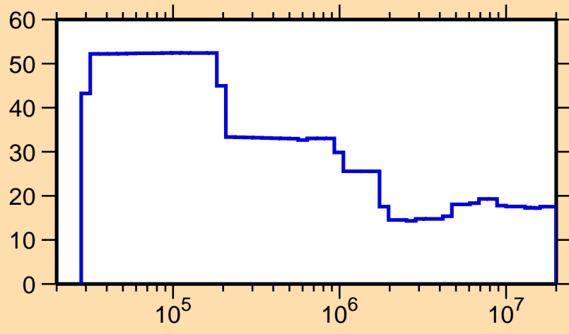
\Delta\sigma/\sigma vs. E for ^{150}\text{Ho}(n,\text{nonel.})
