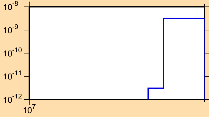
\sigma vs. E for ^{150}\text{Ho}(n,nt)
