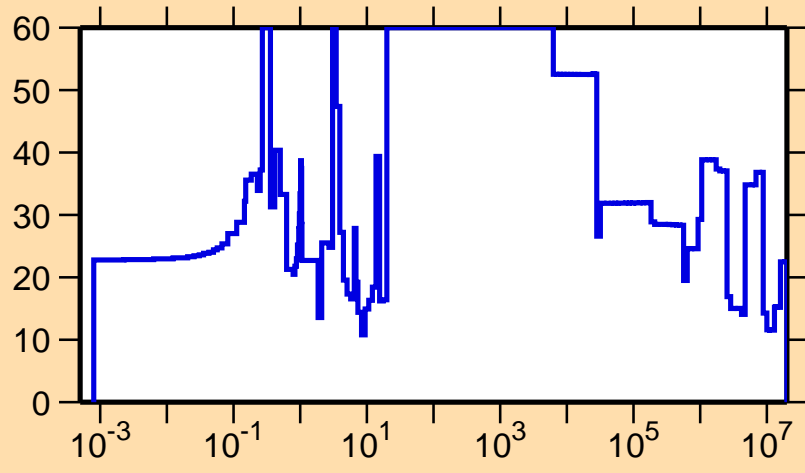
\Delta\sigma/\sigma vs. E for ^{150}\text{Ho}(n,\text{el.})
