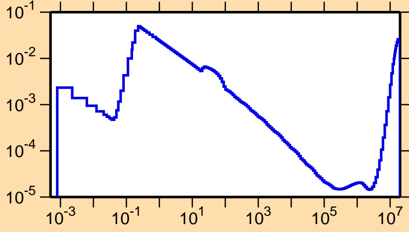
\sigma vs. E for ^{150}\text{Ho}(n,p\alpha)
