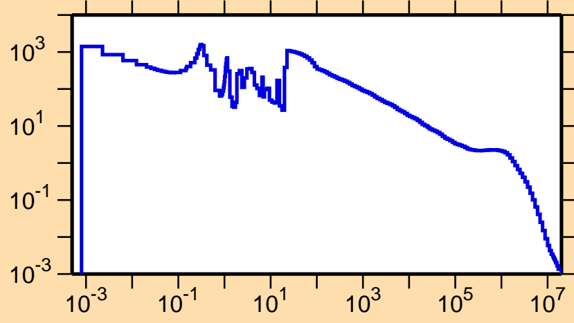
\sigma vs. E for ^{150}\text{Ho}(n,\gamma)
