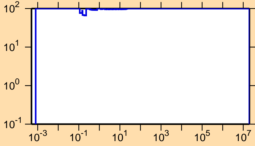
\Delta\sigma/\sigma vs. E for ^{150}\text{Ho}(n,p)
