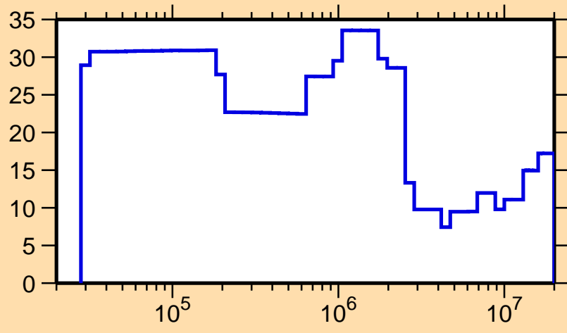
\Delta\sigma/\sigma vs. E for ^{150}\text{Ho}(n,\text{tot.})
