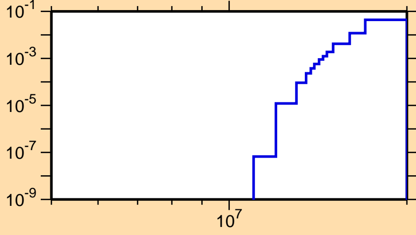
\sigma vs. E for ^{150}\text{Ho}(n,2np)
