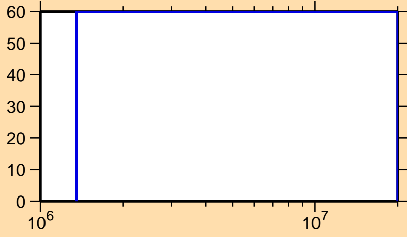
\Delta\sigma/\sigma vs. E for ^{150}\text{Ho}(n,n\text{cont.})
