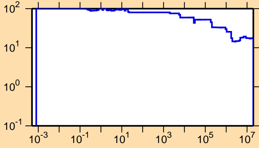
\Delta\sigma/\sigma vs. E for ^{150}\text{Ho}(n,\text{nonel.})
